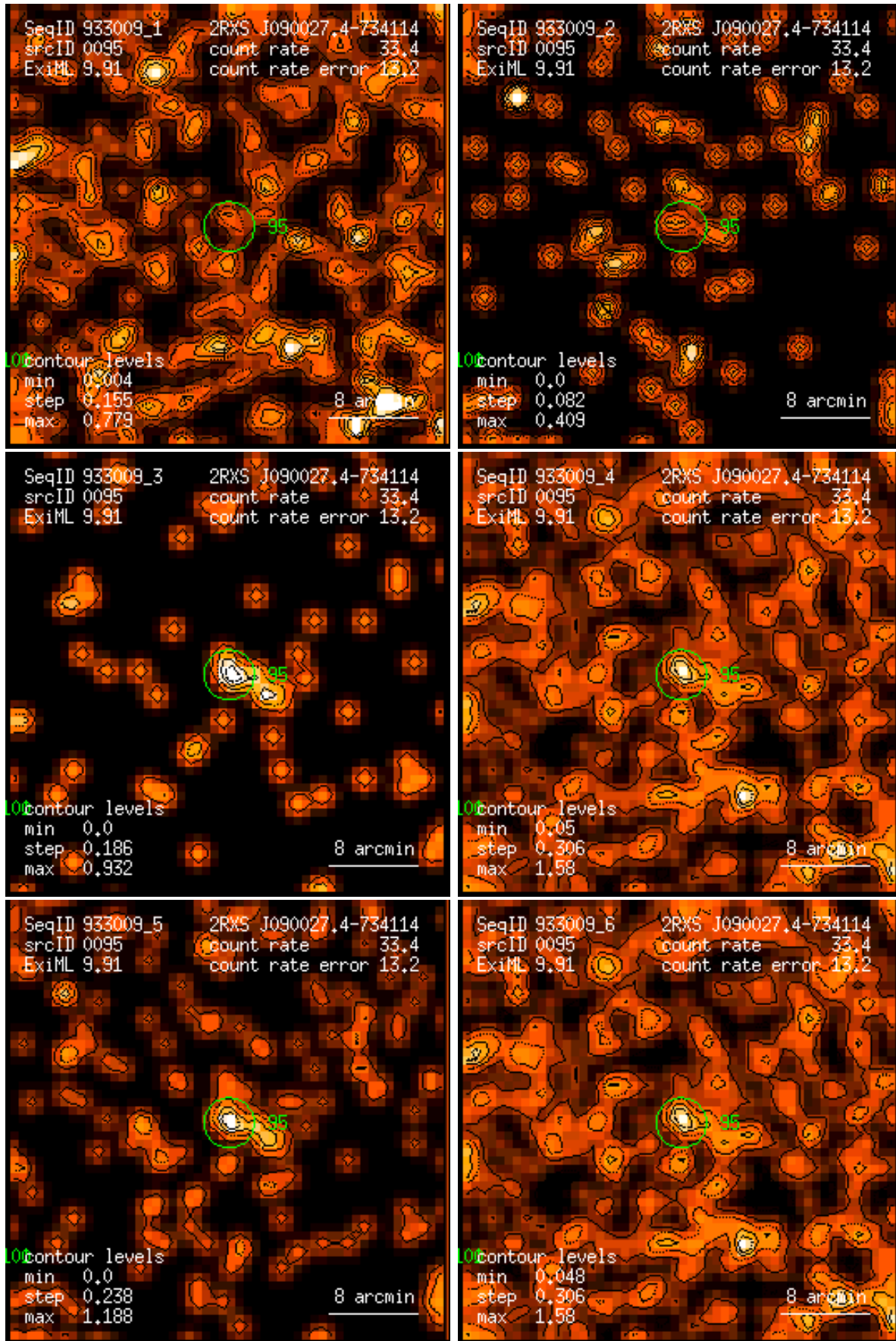
Figure 95: RASS 933009: detection 0095: band rate images, Gaussian filter: (1) PSPC channels 11 – 41, (2) 52 – 90, (3) 91 – 201, (4) 11 – 235, (5) 52 – 201, (6) 11 – 201. Broad band rates in counts/ks. Band rate contour levels in counts/ks/arcmin 2 .
