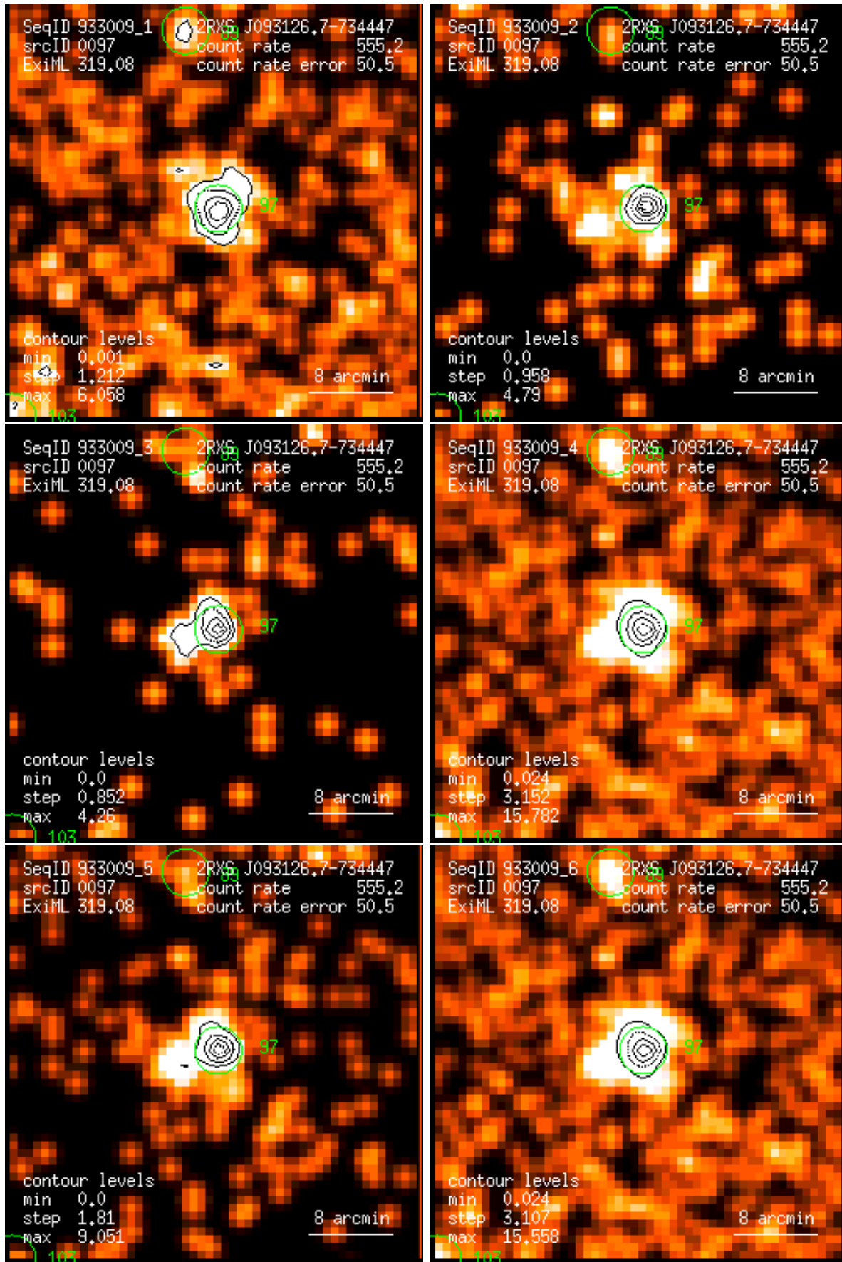
Figure 97: RASS 933009: detection 0097: band rate images, Gaussian filter: (1) PSPC channels 11 – 41, (2) 52 – 90, (3) 91 – 201, (4) 11 – 235, (5) 52 – 201, (6) 11 – 201. Broad band rates in counts/ks. Band rate contour levels in counts/ks/arcmin 2 .
