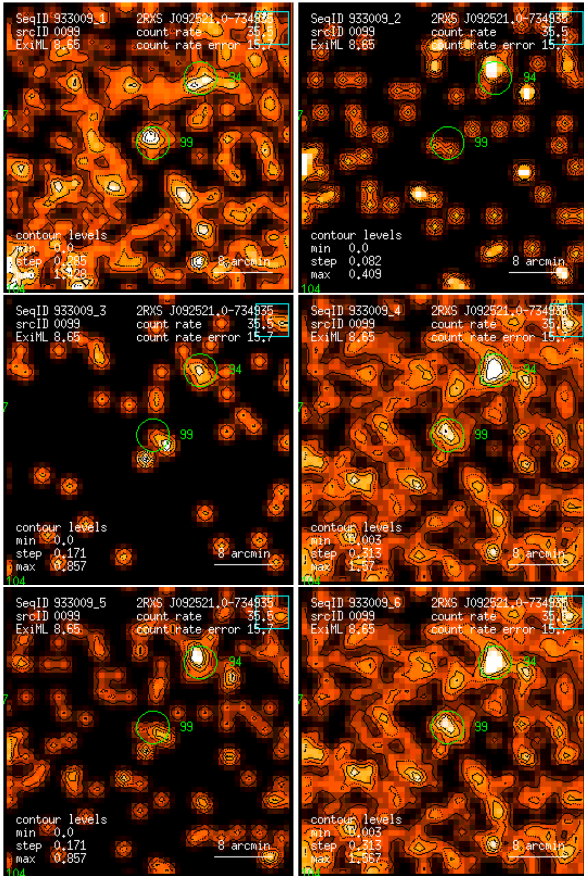
Figure 99: RASS 933009: detection 0099: band rate images, Gaussian filter: (1) PSPC channels 11 – 41, (2) 52 – 90, (3) 91 – 201, (4) 11 – 235, (5) 52 – 201, (6) 11 – 201. Broad band rates in counts/ks. Band rate contour levels in counts/ks/arcmin 2 .
