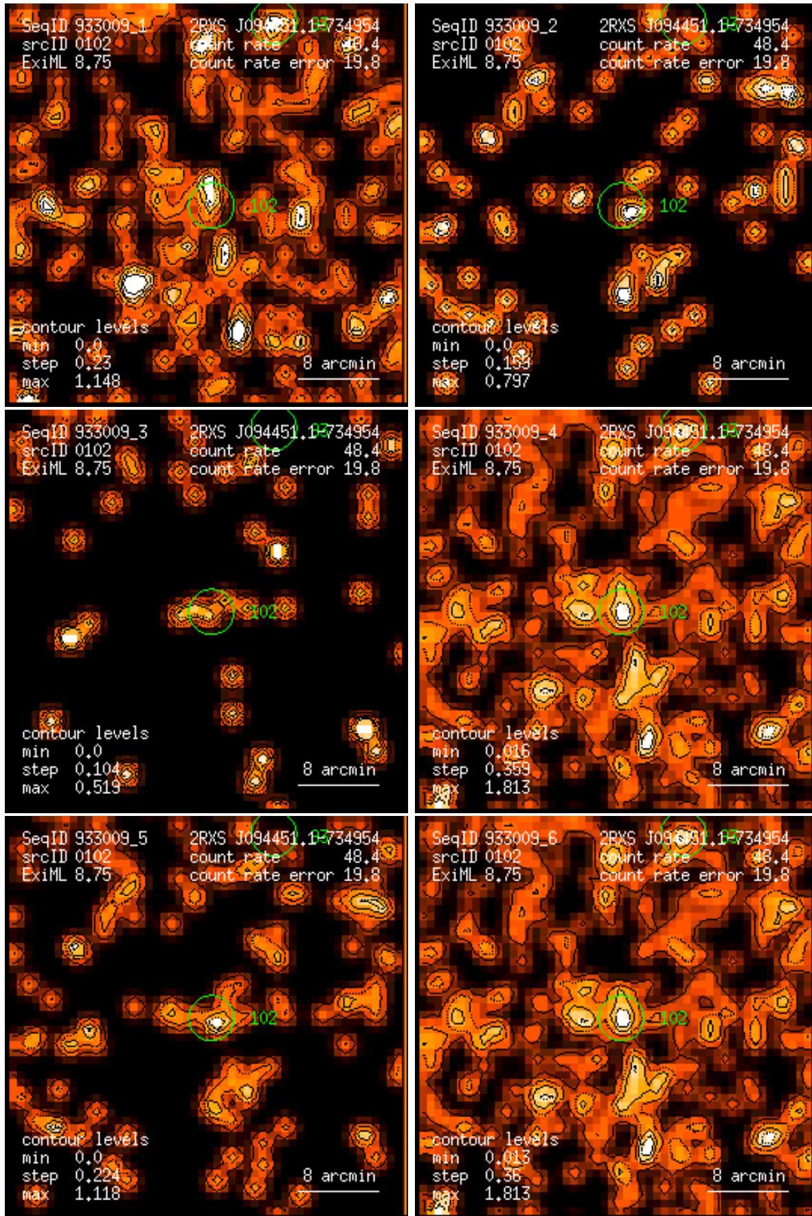
Figure 102: RASS 933009: detection 0102: band rate images, Gaussian filter: (1) PSPC channels 11 – 41, (2) 52 – 90, (3) 91 – 201, (4) 11 – 235, (5) 52 – 201, (6) 11 – 201. Broad band rates in counts/ks. Band rate contour levels in counts/ks/arcmin 2 .
