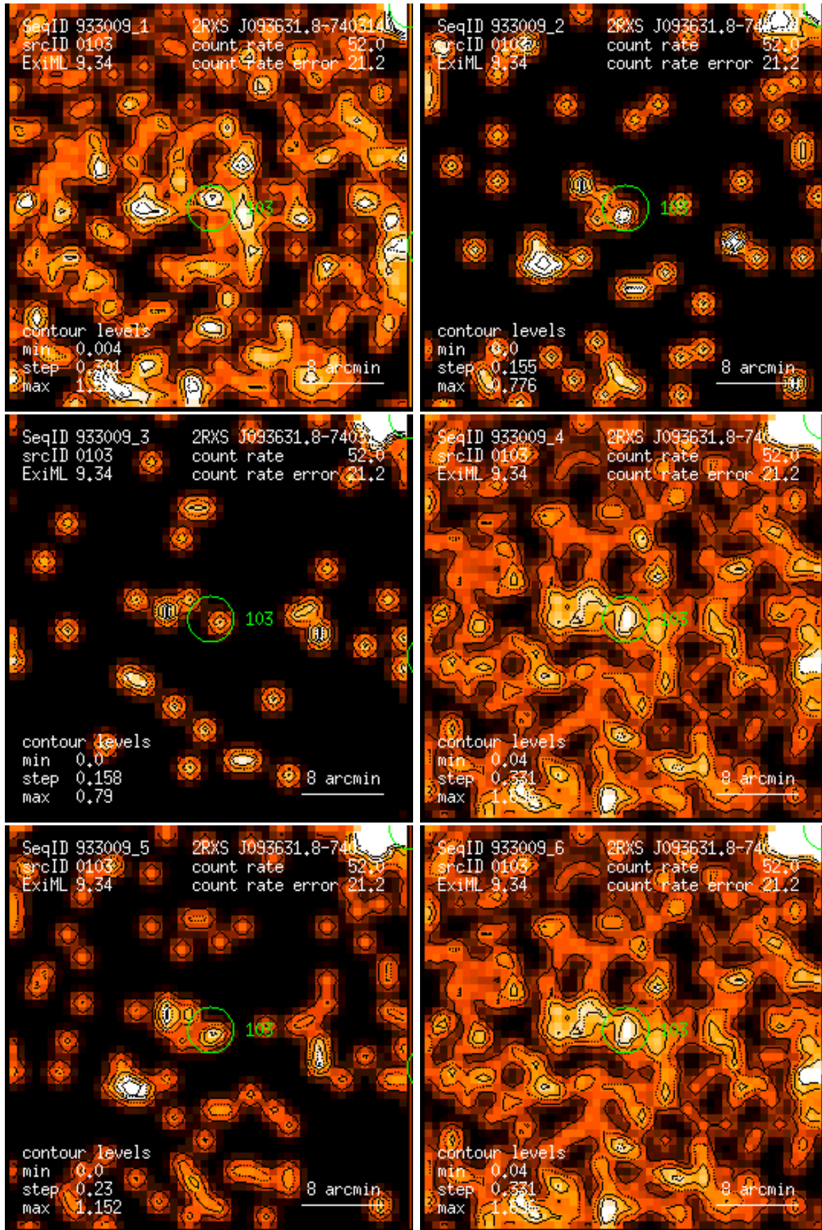
Figure 103: RASS 933009: detection 0103: band rate images, Gaussian filter: (1) PSPC channels 11 – 41, (2) 52 – 90, (3) 91 – 201, (4) 11 – 235, (5) 52 – 201, (6) 11 – 201. Broad band rates in counts/ks. Band rate contour levels in counts/ks/arcmin 2 .
