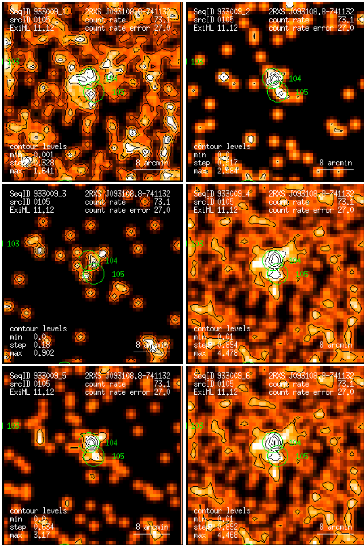
Figure 105: RASS 933009: detection 0105: band rate images, Gaussian filter: (1) PSPC channels 11 – 41, (2) 52 – 90, (3) 91 – 201, (4) 11 – 235, (5) 52 – 201, (6) 11 – 201. Broad band rates in counts/ks. Band rate contour levels in counts/ks/arcmin 2 .
