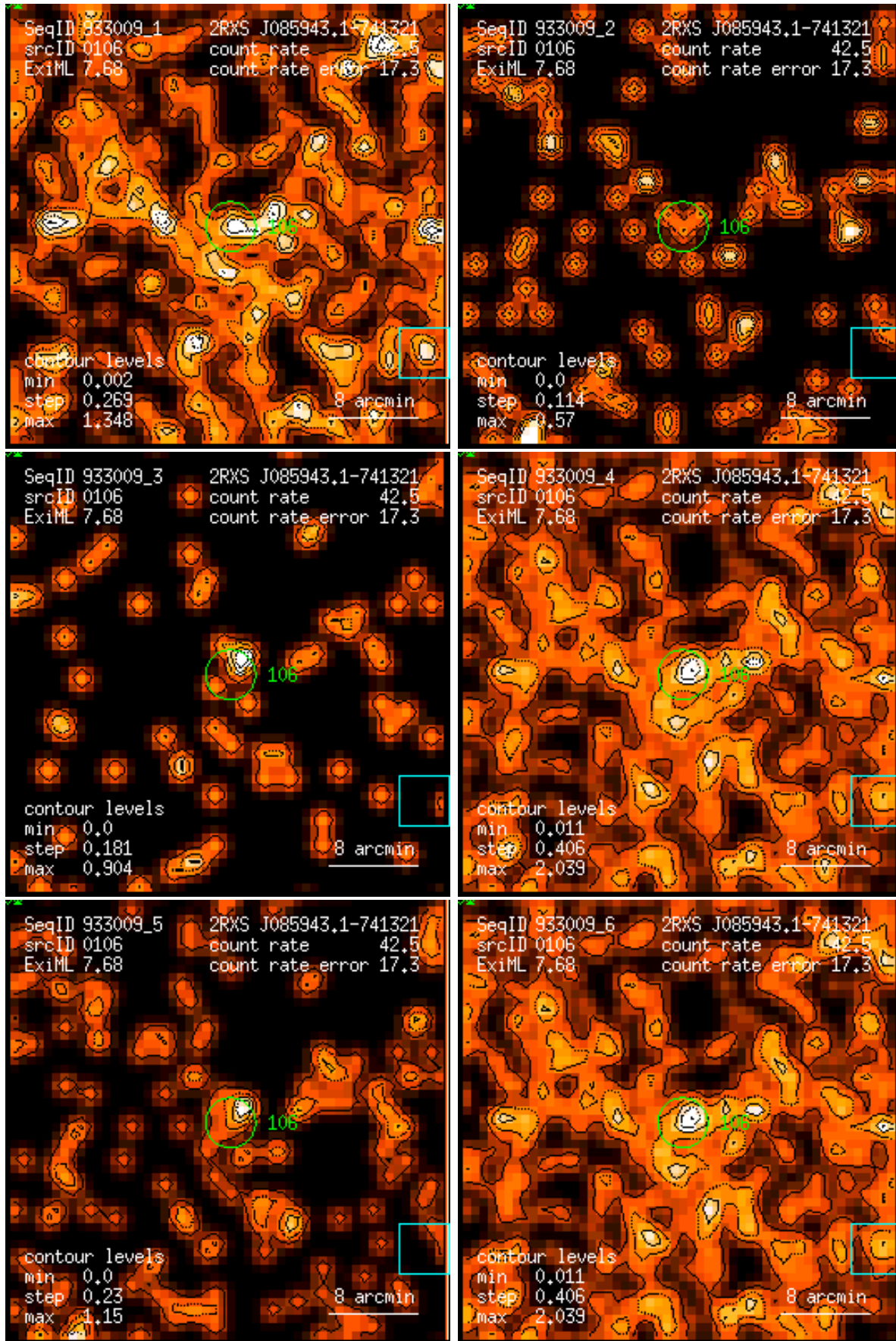
Figure 106: RASS 933009: detection 0106: band rate images, Gaussian filter: (1) PSPC channels 11 – 41, (2) 52 – 90, (3) 91 – 201, (4) 11 – 235, (5) 52 – 201, (6) 11 – 201. Broad band rates in counts/ks. Band rate contour levels in counts/ks/arcmin 2 .
