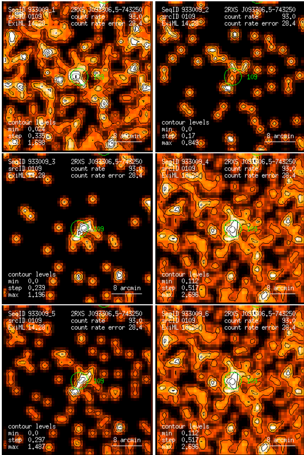
Figure 109: RASS 933009: detection 0109: band rate images, Gaussian filter: (1) PSPC channels 11 – 41, (2) 52 – 90, (3) 91 – 201, (4) 11 – 235, (5) 52 – 201, (6) 11 – 201. Broad band rates in counts/ks. Band rate contour levels in counts/ks/arcmin 2 .
