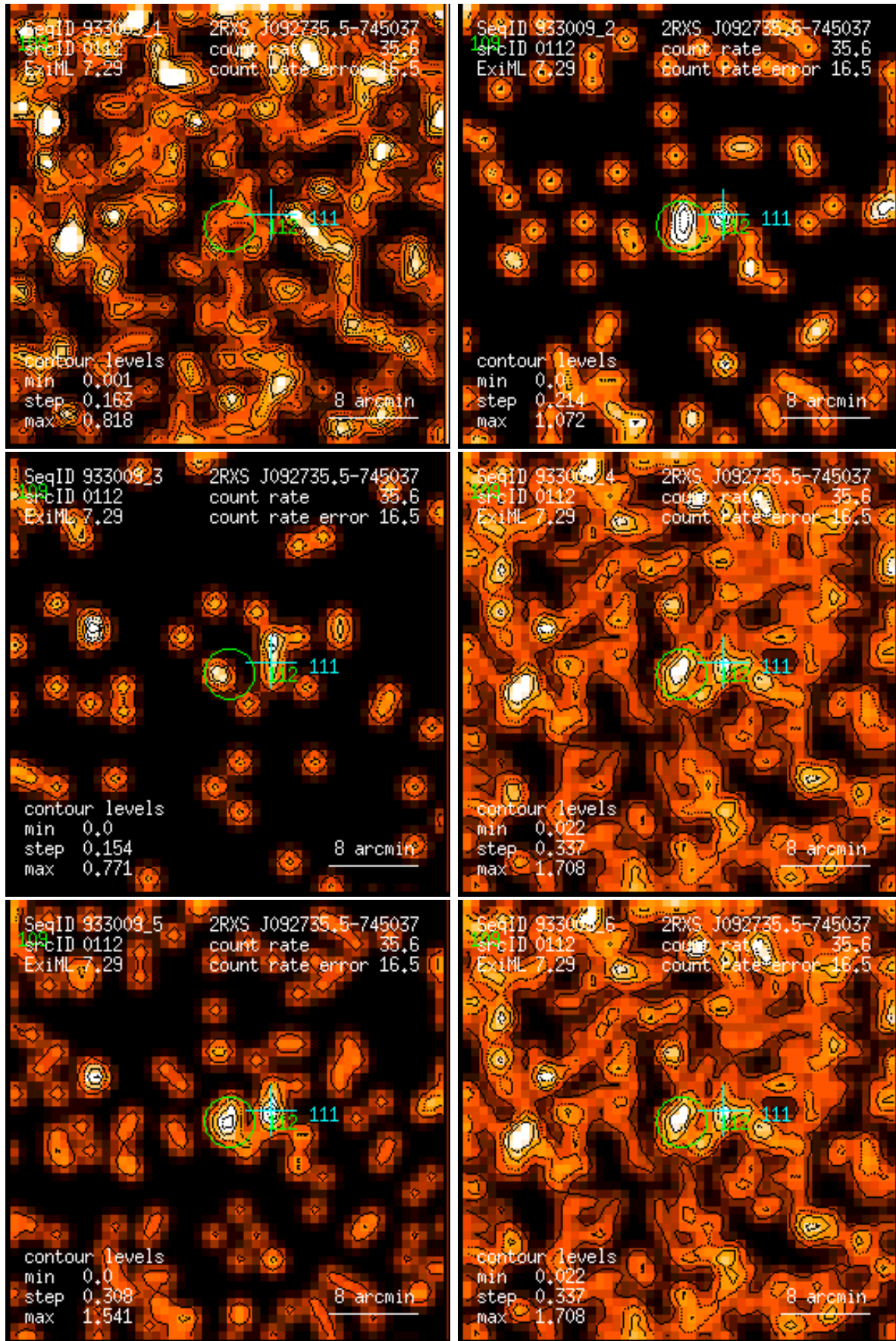
Figure 112: RASS 933009: detection 0112: band rate images, Gaussian filter: (1) PSPC channels 11 – 41, (2) 52 – 90, (3) 91 – 201, (4) 11 – 235, (5) 52 – 201, (6) 11 – 201. Broad band rates in counts/ks. Band rate contour levels in counts/ks/arcmin 2 .
