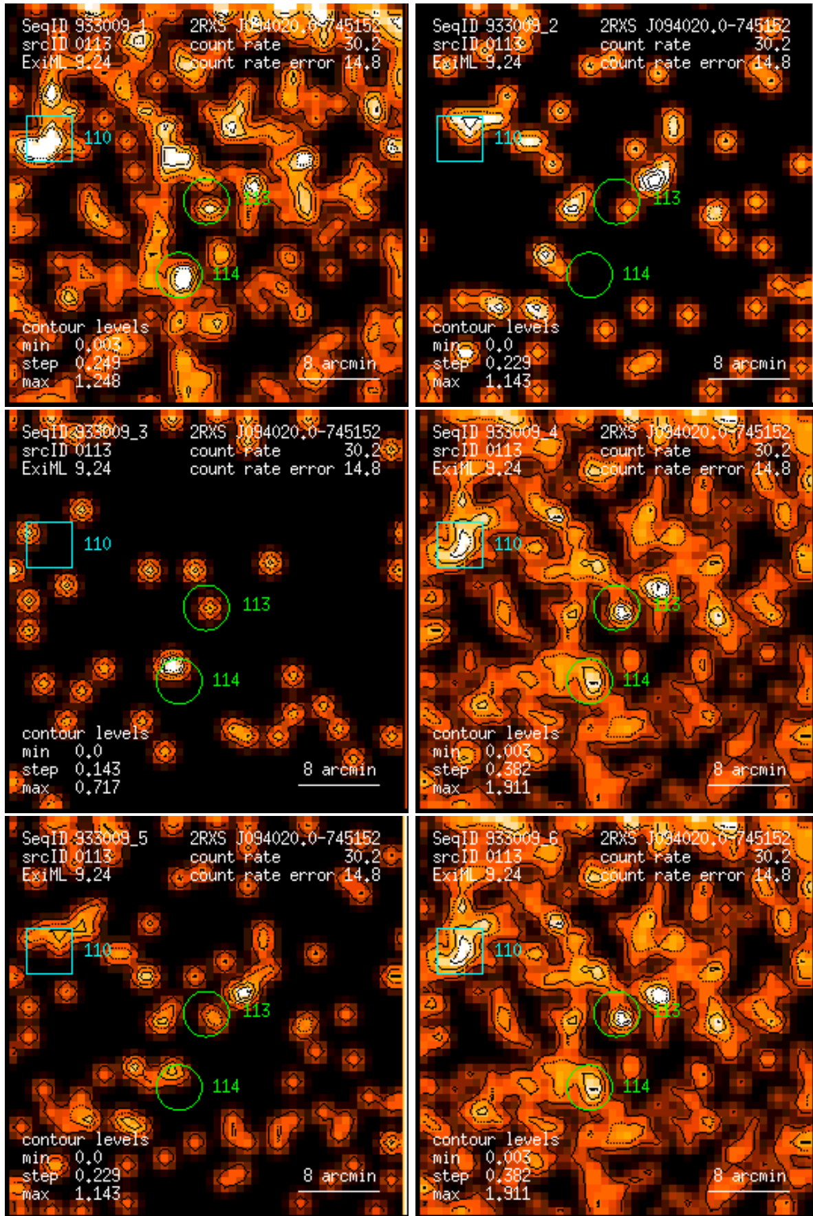
Figure 113: RASS 933009: detection 0113: band rate images, Gaussian filter: (1) PSPC channels 11 – 41, (2) 52 – 90, (3) 91 – 201, (4) 11 – 235, (5) 52 – 201, (6) 11 – 201. Broad band rates in counts/ks. Band rate contour levels in counts/ks/arcmin 2 .
