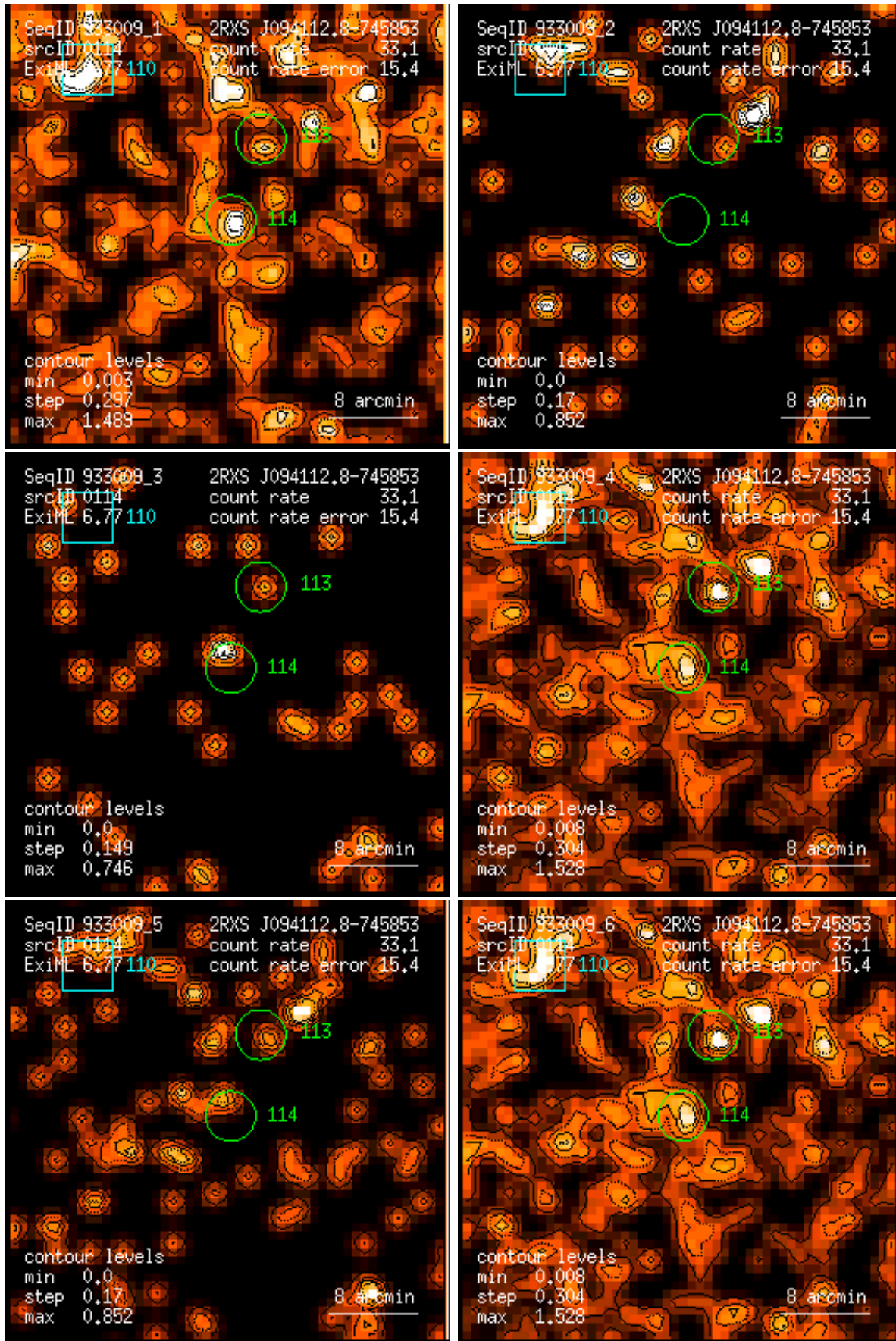
Figure 114: RASS 933009: detection 0114: band rate images, Gaussian filter: (1) PSPC channels 11 – 41, (2) 52 – 90, (3) 91 – 201, (4) 11 – 235, (5) 52 – 201, (6) 11 – 201. Broad band rates in counts/ks. Band rate contour levels in counts/ks/arcmin 2 .
