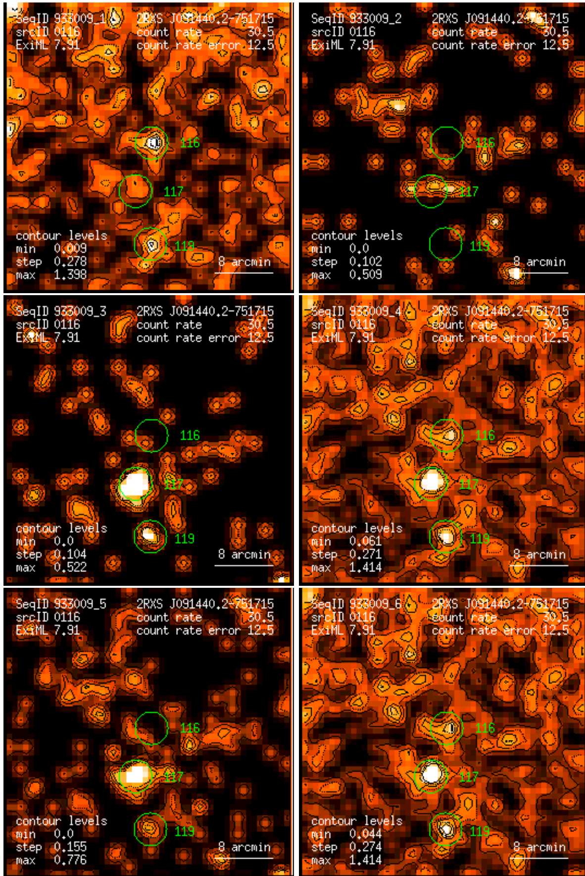
Figure 116: RASS 933009: detection 0116: band rate images, Gaussian filter: (1) PSPC channels 11 – 41, (2) 52 – 90, (3) 91 – 201, (4) 11 – 235, (5) 52 – 201, (6) 11 – 201. Broad band rates in counts/ks. Band rate contour levels in counts/ks/arcmin 2 .
