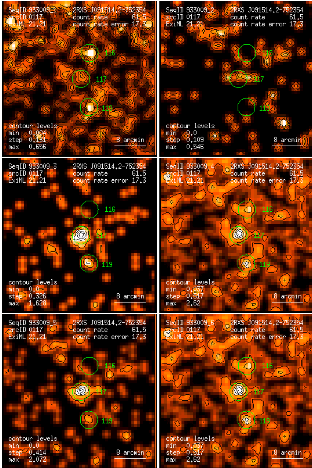
Figure 117: RASS 933009: detection 0117: band rate images, Gaussian filter: (1) PSPC channels 11 – 41, (2) 52 – 90, (3) 91 – 201, (4) 11 – 235, (5) 52 – 201, (6) 11 – 201. Broad band rates in counts/ks. Band rate contour levels in counts/ks/arcmin 2 .
