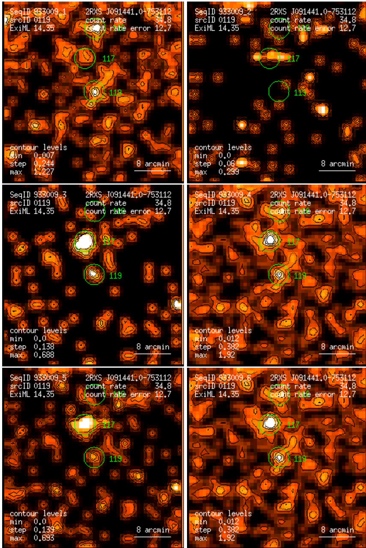
Figure 119: RASS 933009: detection 0119: band rate images, Gaussian filter: (1) PSPC channels 11 – 41, (2) 52 – 90, (3) 91 – 201, (4) 11 – 235, (5) 52 – 201, (6) 11 – 201. Broad band rates in counts/ks. Band rate contour levels in counts/ks/arcmin 2 .
