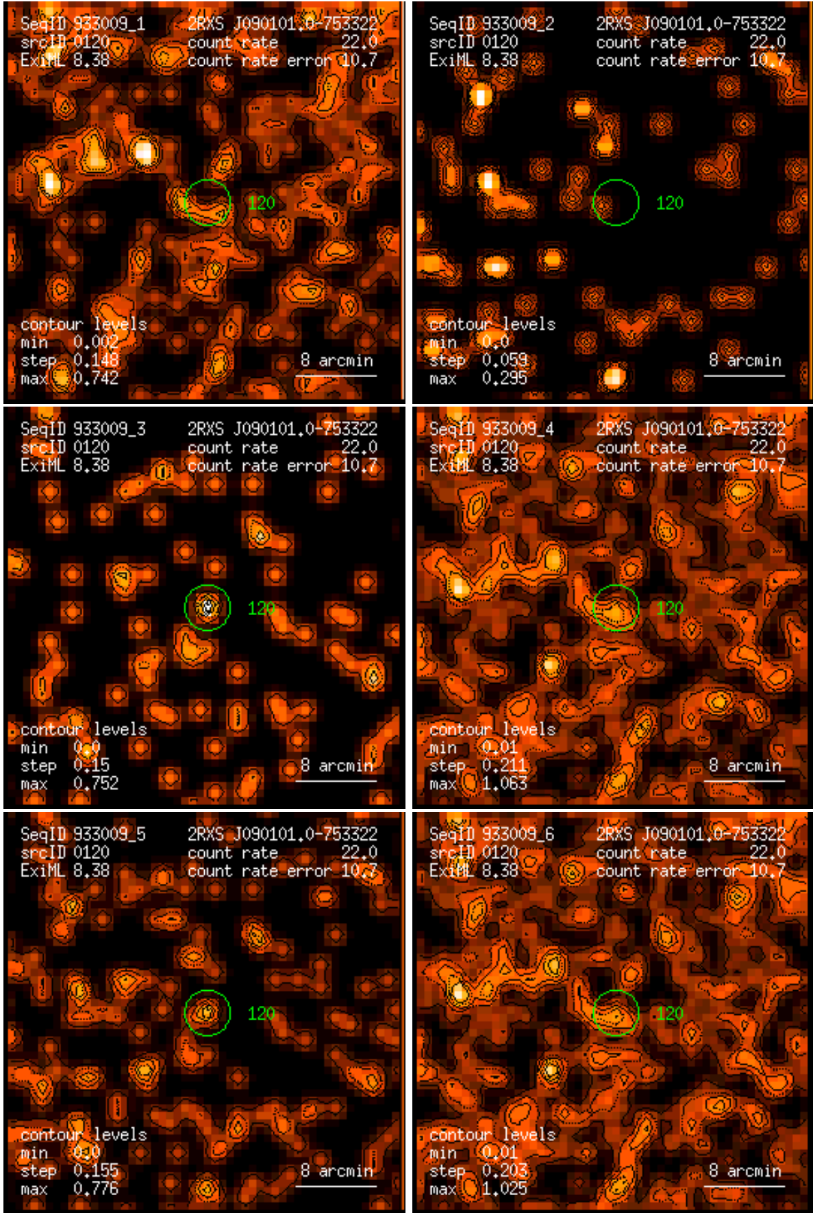
Figure 120: RASS 933009: detection 0120: band rate images, Gaussian filter: (1) PSPC channels 11 – 41, (2) 52 – 90, (3) 91 – 201, (4) 11 – 235, (5) 52 – 201, (6) 11 – 201. Broad band rates in counts/ks. Band rate contour levels in counts/ks/arcmin 2 .
