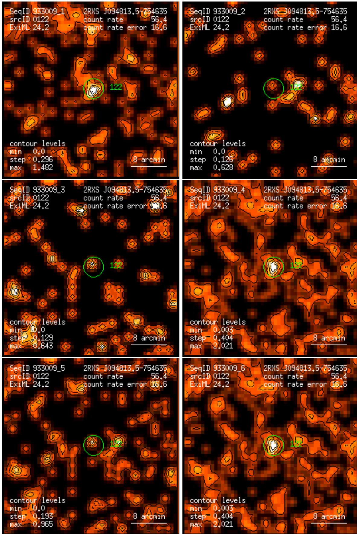
Figure 122: RASS 933009: detection 0122: band rate images, Gaussian filter: (1) PSPC channels 11 – 41, (2) 52 – 90, (3) 91 – 201, (4) 11 – 235, (5) 52 – 201, (6) 11 – 201. Broad band rates in counts/ks. Band rate contour levels in counts/ks/arcmin 2 .
