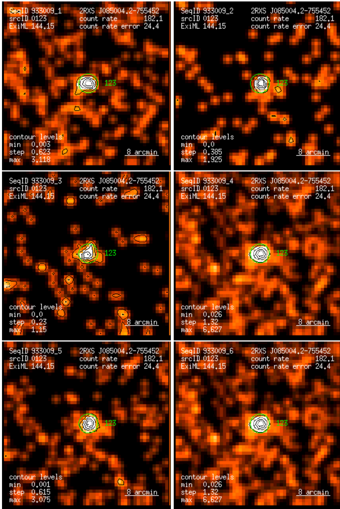
Figure 123: RASS 933009: detection 0123: band rate images, Gaussian filter: (1) PSPC channels 11 – 41, (2) 52 – 90, (3) 91 – 201, (4) 11 – 235, (5) 52 – 201, (6) 11 – 201. Broad band rates in counts/ks. Band rate contour levels in counts/ks/arcmin 2 .
