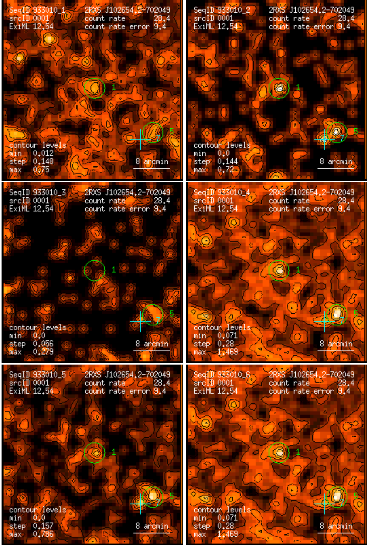
Figure 1: RASS 933010: detection 0001: band rate images, Gaussian filter: (1) PSPC channels 11 – 41, (2) 52 – 90, (3) 91 – 201, (4) 11 – 235, (5) 52 – 201, (6) 11 – 201. Broad band rates in counts/ks. Band rate contour levels in counts/ks/arcmin 2 .
