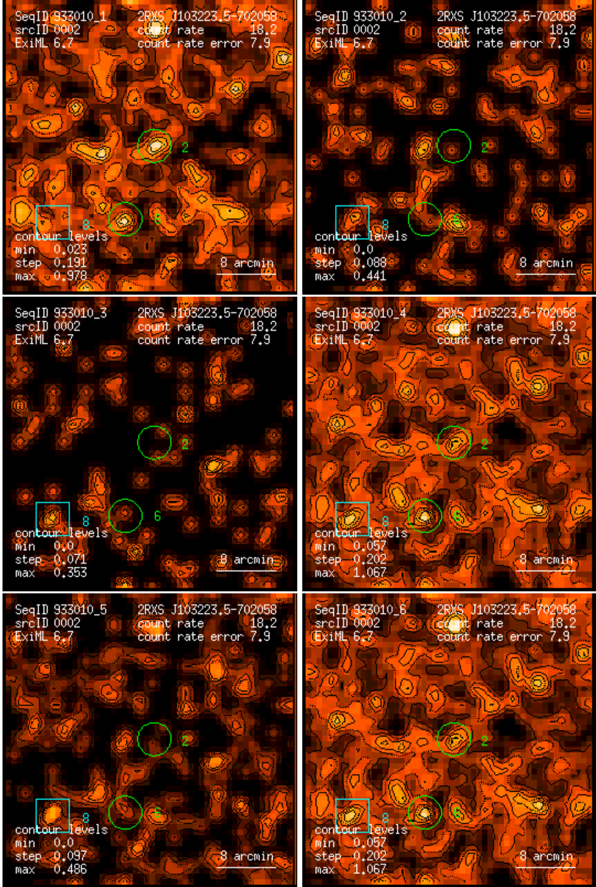
Figure 2: RASS 933010: detection 0002: band rate images, Gaussian filter: (1) PSPC channels 11 – 41, (2) 52 – 90, (3) 91 – 201, (4) 11 – 235, (5) 52 – 201, (6) 11 – 201. Broad band rates in counts/ks. Band rate contour levels in counts/ks/arcmin 2 .
