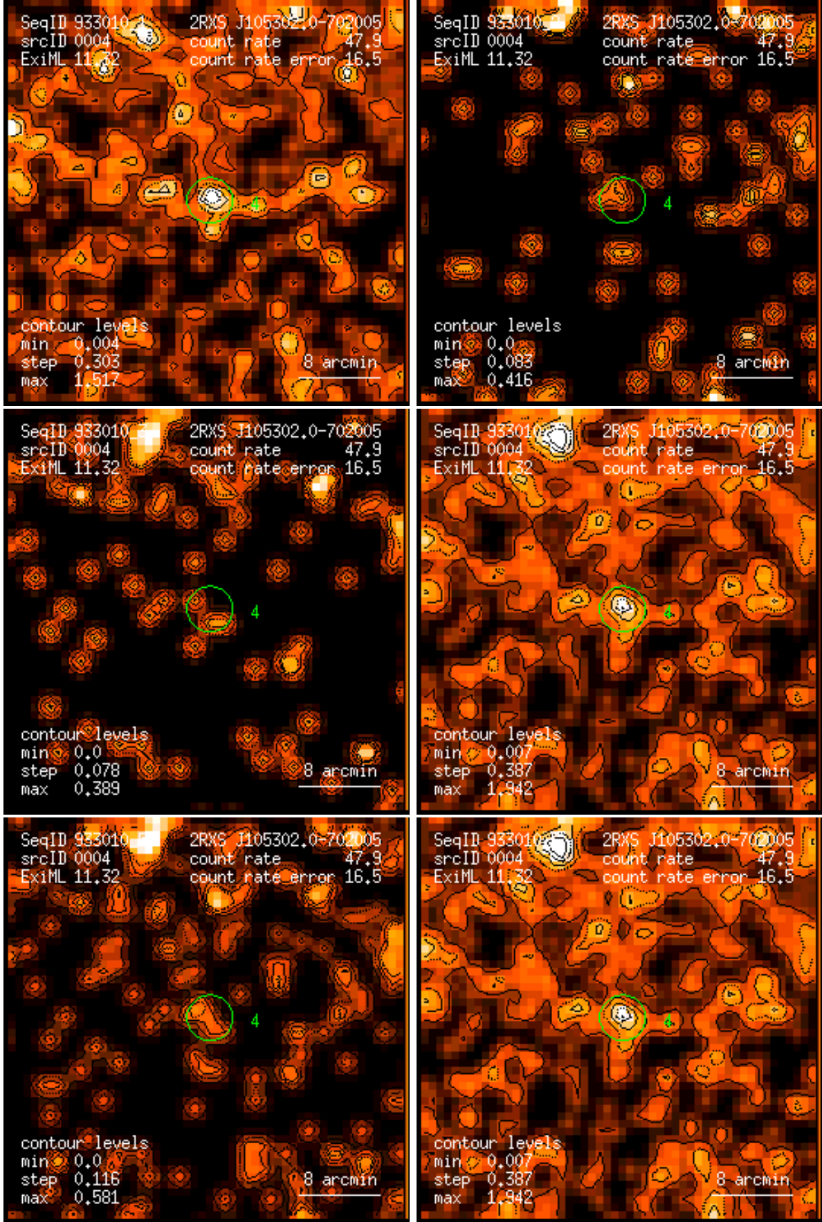
Figure 4: RASS 933010: detection 0004: band rate images, Gaussian filter: (1) PSPC channels 11 – 41, (2) 52 – 90, (3) 91 – 201, (4) 11 – 235, (5) 52 – 201, (6) 11 – 201. Broad band rates in counts/ks. Band rate contour levels in counts/ks/arcmin 2 .
