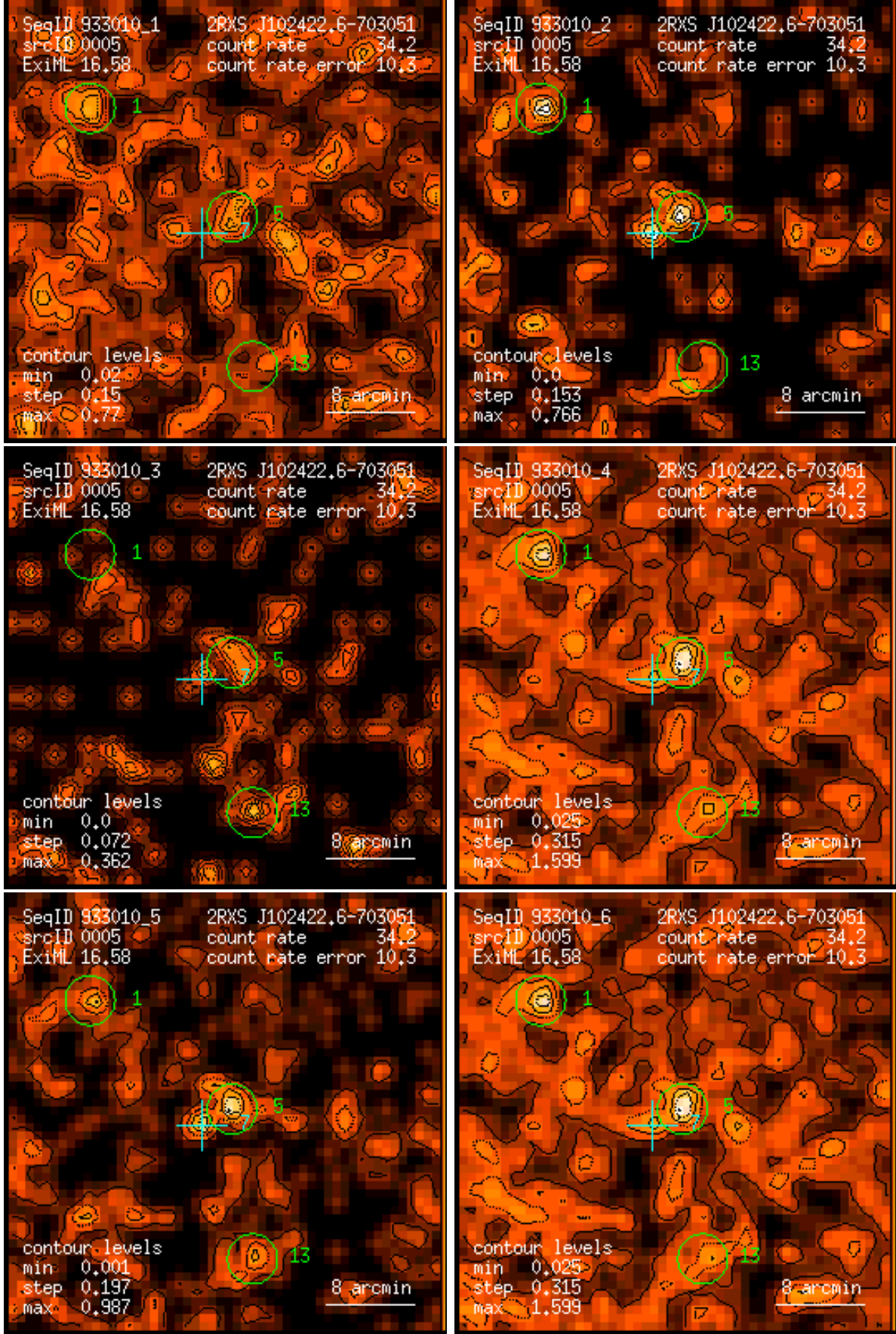
Figure 5: RASS 933010: detection 0005: band rate images, Gaussian filter: (1) PSPC channels 11 – 41, (2) 52 – 90, (3) 91 – 201, (4) 11 – 235, (5) 52 – 201, (6) 11 – 201. Broad band rates in counts/ks. Band rate contour levels in counts/ks/arcmin 2 .
