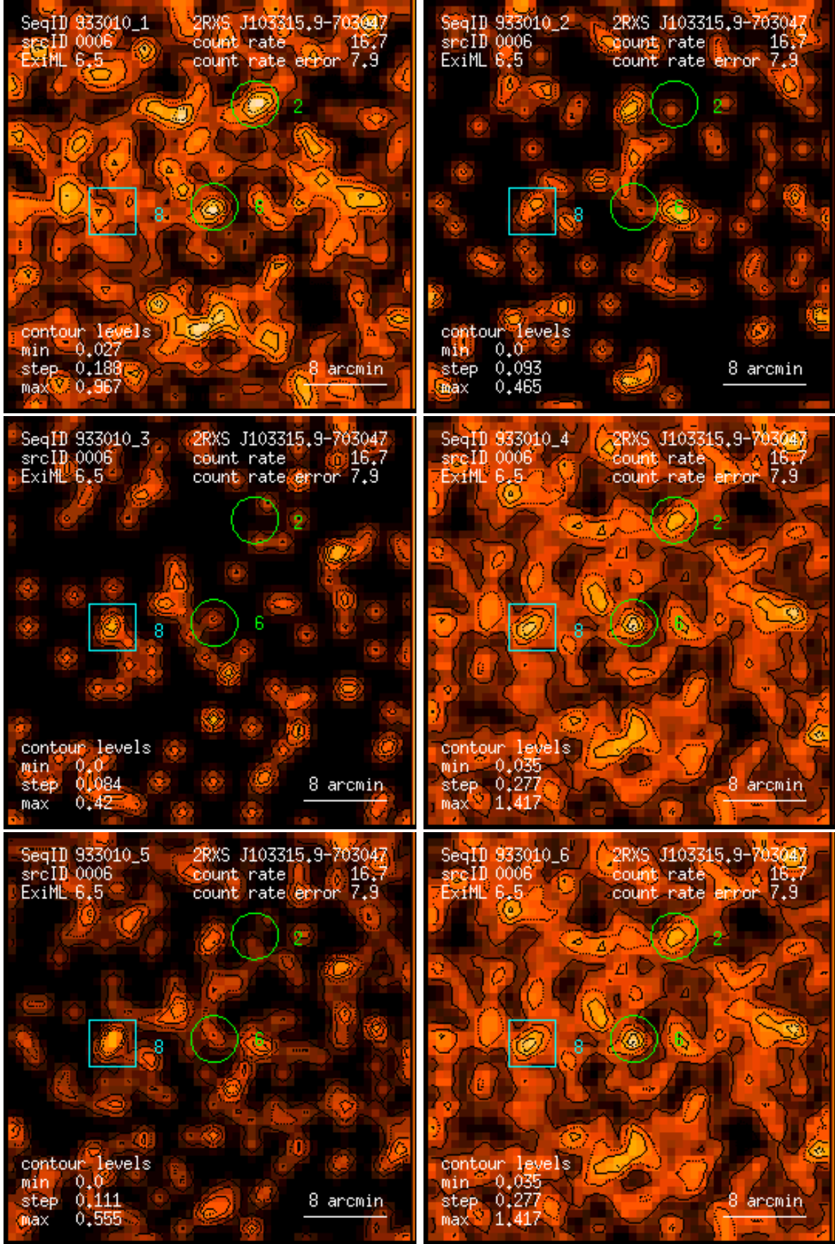
Figure 6: RASS 933010: detection 0006: band rate images, Gaussian filter: (1) PSPC channels 11 – 41, (2) 52 – 90, (3) 91 – 201, (4) 11 – 235, (5) 52 – 201, (6) 11 – 201. Broad band rates in counts/ks. Band rate contour levels in counts/ks/arcmin 2 .
