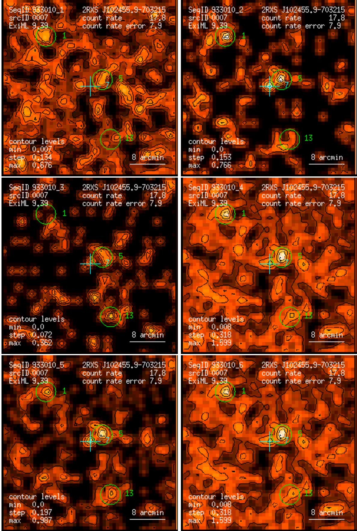
Figure 7: RASS 933010: detection 0007: band rate images, Gaussian filter: (1) PSPC channels 11 – 41, (2) 52 – 90, (3) 91 – 201, (4) 11 – 235, (5) 52 – 201, (6) 11 – 201. Broad band rates in counts/ks. Band rate contour levels in counts/ks/arcmin 2 .
