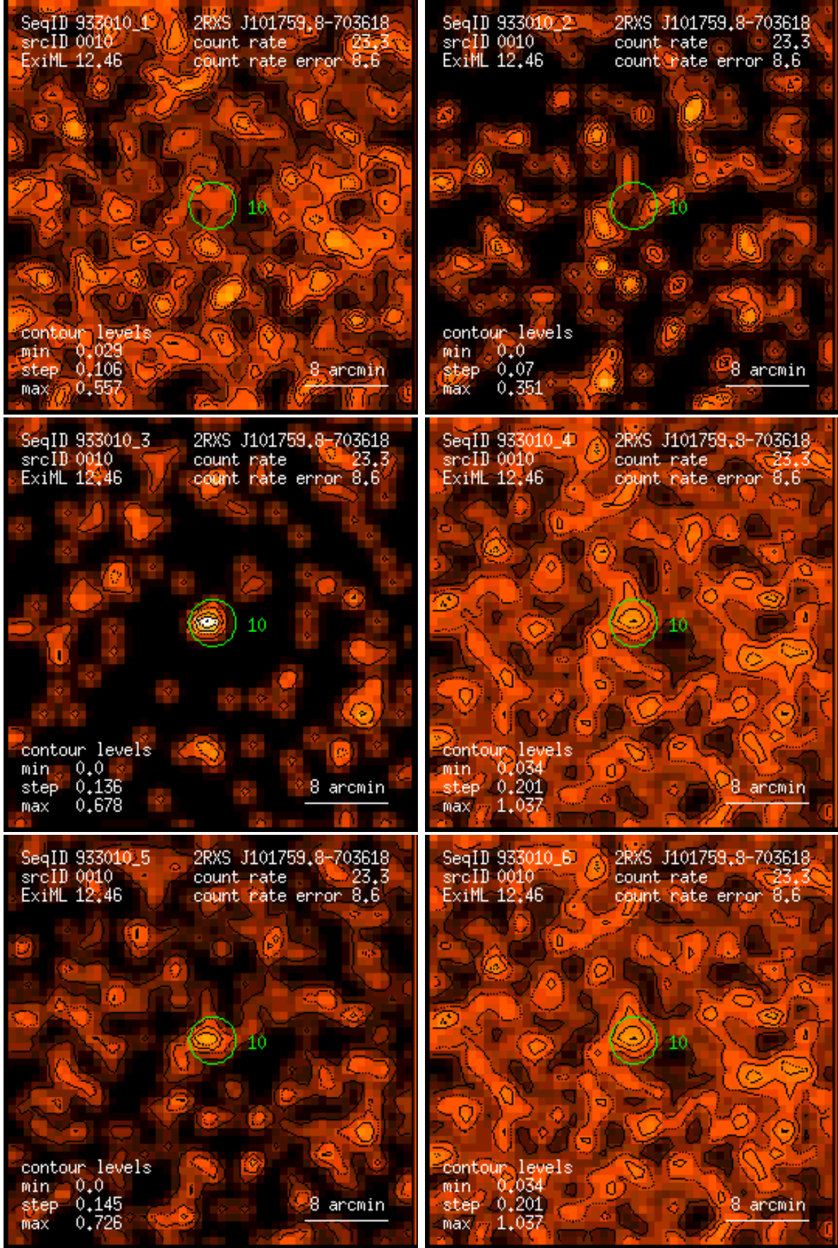
Figure 10: RASS 933010: detection 0010: band rate images, Gaussian filter: (1) PSPC channels 11 – 41, (2) 52 – 90, (3) 91 – 201, (4) 11 – 235, (5) 52 – 201, (6) 11 – 201. Broad band rates in counts/ks. Band rate contour levels in counts/ks/arcmin 2 .
