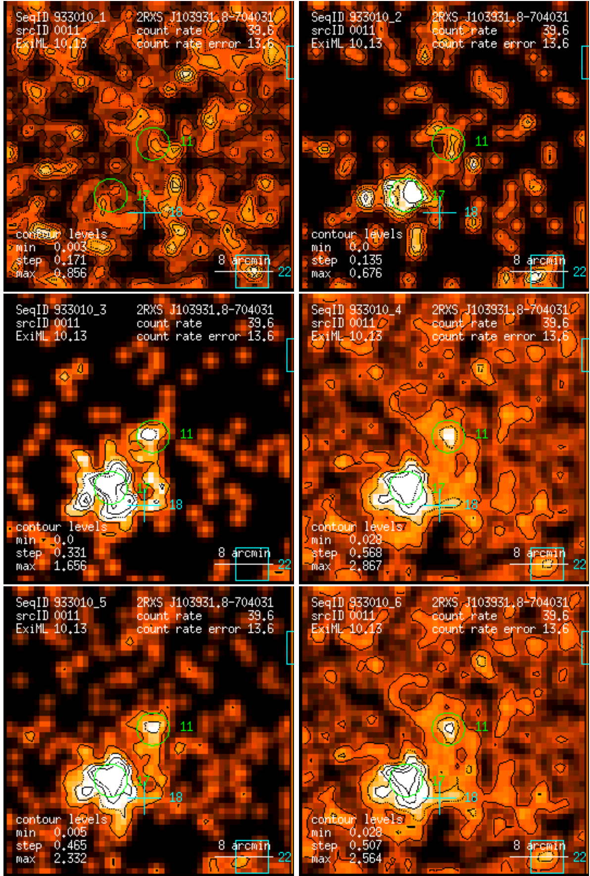
Figure 11: RASS 933010: detection 0011: band rate images, Gaussian filter: (1) PSPC channels 11 – 41, (2) 52 – 90, (3) 91 – 201, (4) 11 – 235, (5) 52 – 201, (6) 11 – 201. Broad band rates in counts/ks. Band rate contour levels in counts/ks/arcmin 2 .
