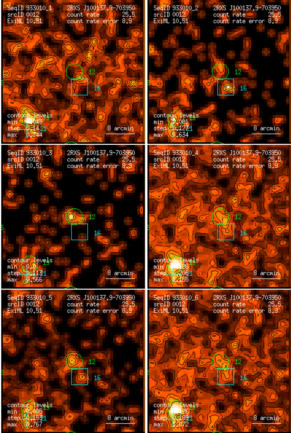
Figure 12: RASS 933010: detection 0012: band rate images, Gaussian filter: (1) PSPC channels 11 – 41, (2) 52 – 90, (3) 91 – 201, (4) 11 – 235, (5) 52 – 201, (6) 11 – 201. Broad band rates in counts/ks. Band rate contour levels in counts/ks/arcmin 2 .
