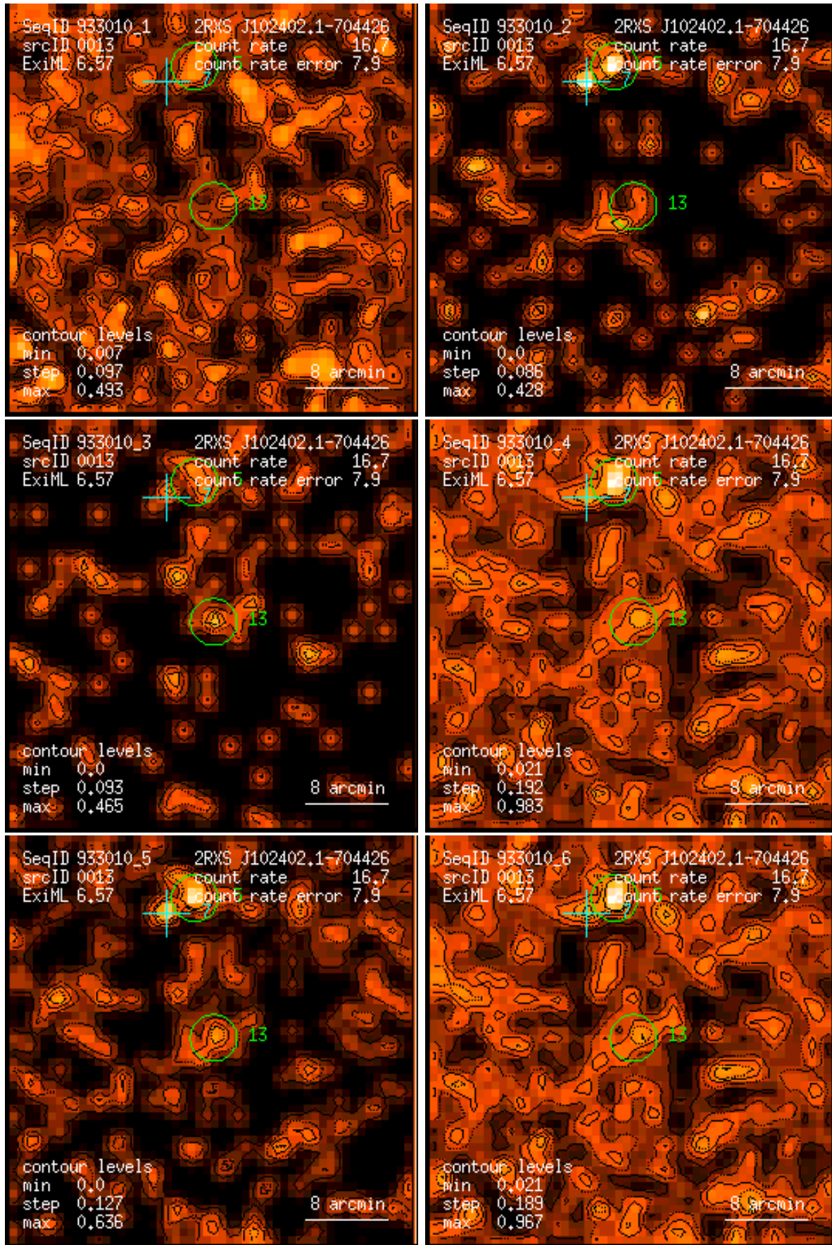
Figure 13: RASS 933010: detection 0013: band rate images, Gaussian filter: (1) PSPC channels 11 – 41, (2) 52 – 90, (3) 91 – 201, (4) 11 – 235, (5) 52 – 201, (6) 11 – 201. Broad band rates in counts/ks. Band rate contour levels in counts/ks/arcmin 2 .
