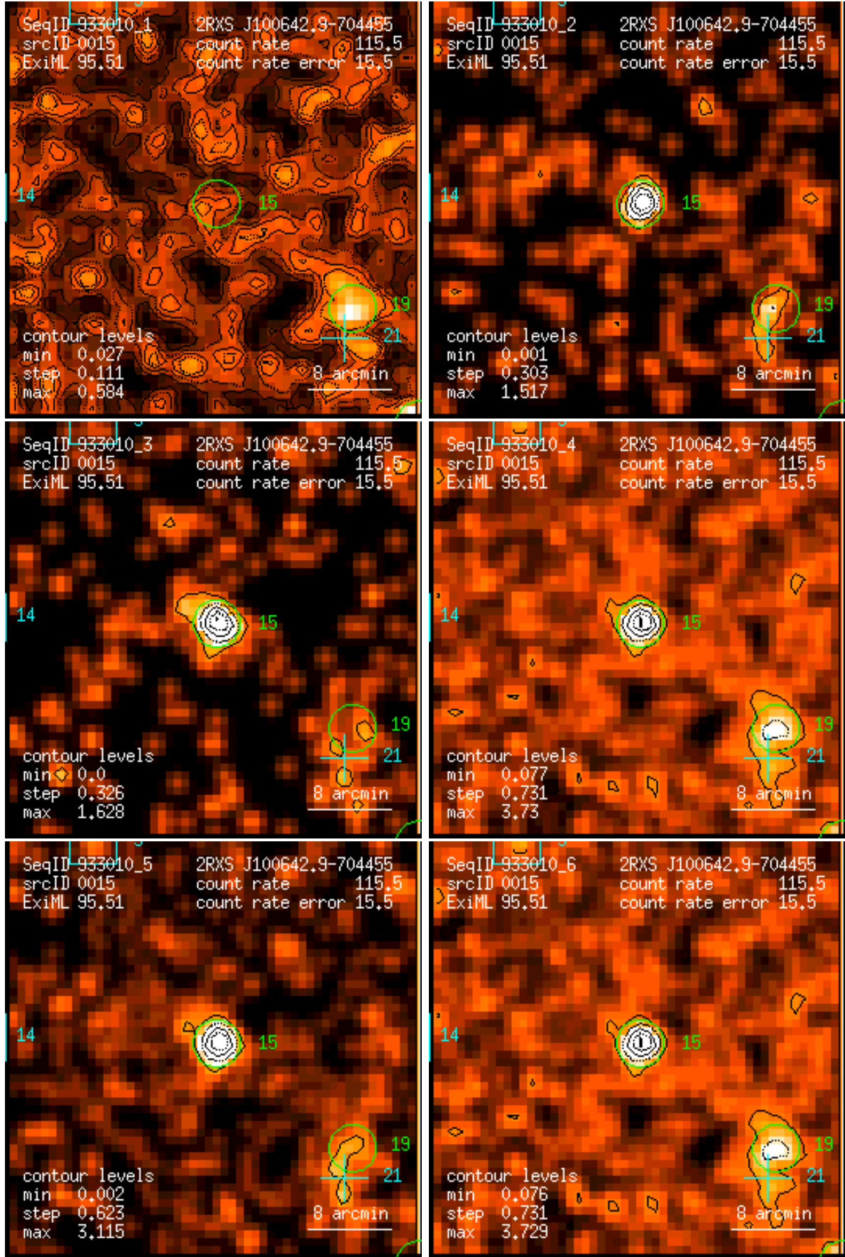
Figure 15: RASS 933010: detection 0015: band rate images, Gaussian filter: (1) PSPC channels 11 – 41, (2) 52 – 90, (3) 91 – 201, (4) 11 – 235, (5) 52 – 201, (6) 11 – 201. Broad band rates in counts/ks. Band rate contour levels in counts/ks/arcmin 2 .
