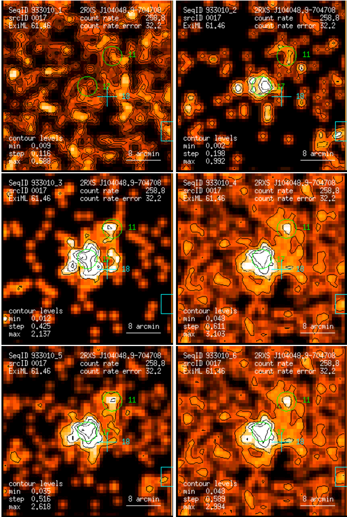
Figure 17: RASS 933010: detection 0017: band rate images, Gaussian filter: (1) PSPC channels 11 – 41, (2) 52 – 90, (3) 91 – 201, (4) 11 – 235, (5) 52 – 201, (6) 11 – 201. Broad band rates in counts/ks. Band rate contour levels in counts/ks/arcmin 2 .
