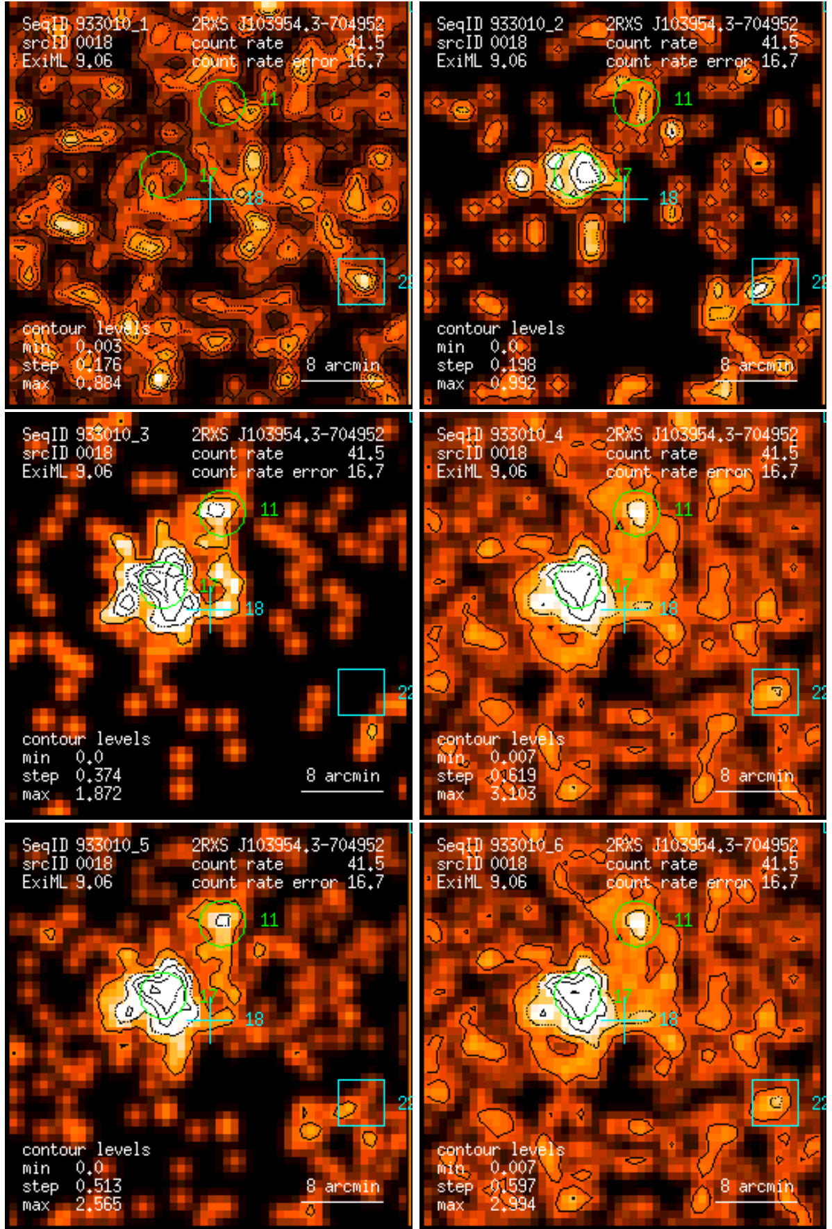
Figure 18: RASS 933010: detection 0018: band rate images, Gaussian filter: (1) PSPC channels 11 – 41, (2) 52 – 90, (3) 91 – 201, (4) 11 – 235, (5) 52 – 201, (6) 11 – 201. Broad band rates in counts/ks. Band rate contour levels in counts/ks/arcmin 2 .
