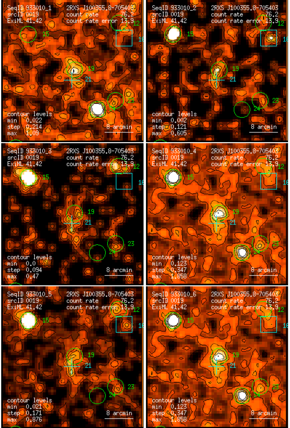
Figure 19: RASS 933010: detection 0019: band rate images, Gaussian filter: (1) PSPC channels 11 – 41, (2) 52 – 90, (3) 91 – 201, (4) 11 – 235, (5) 52 – 201, (6) 11 – 201. Broad band rates in counts/ks. Band rate contour levels in counts/ks/arcmin 2 .
