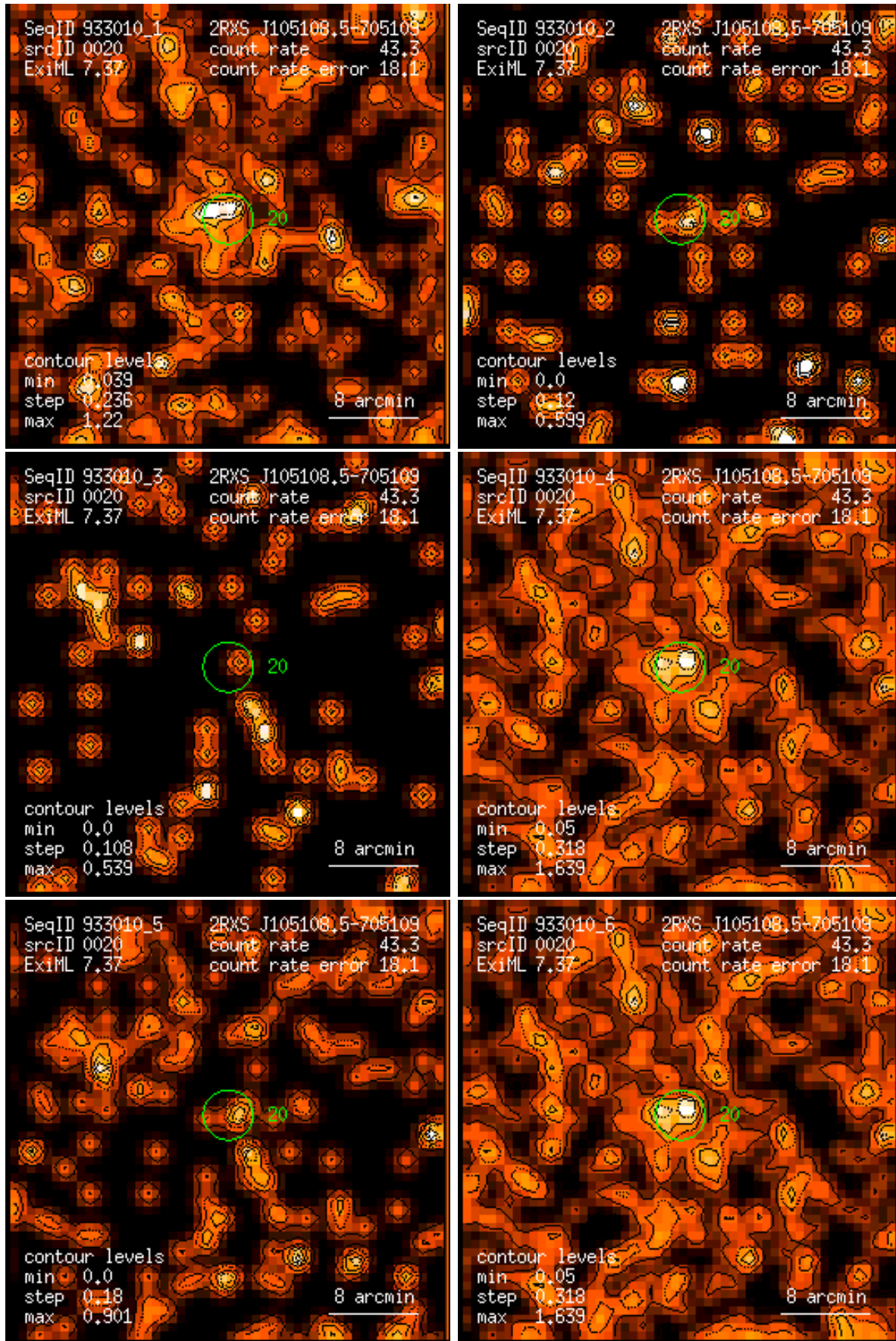
Figure 20: RASS 933010: detection 0020: band rate images, Gaussian filter: (1) PSPC channels 11 – 41, (2) 52 – 90, (3) 91 – 201, (4) 11 – 235, (5) 52 – 201, (6) 11 – 201. Broad band rates in counts/ks. Band rate contour levels in counts/ks/arcmin 2 .
