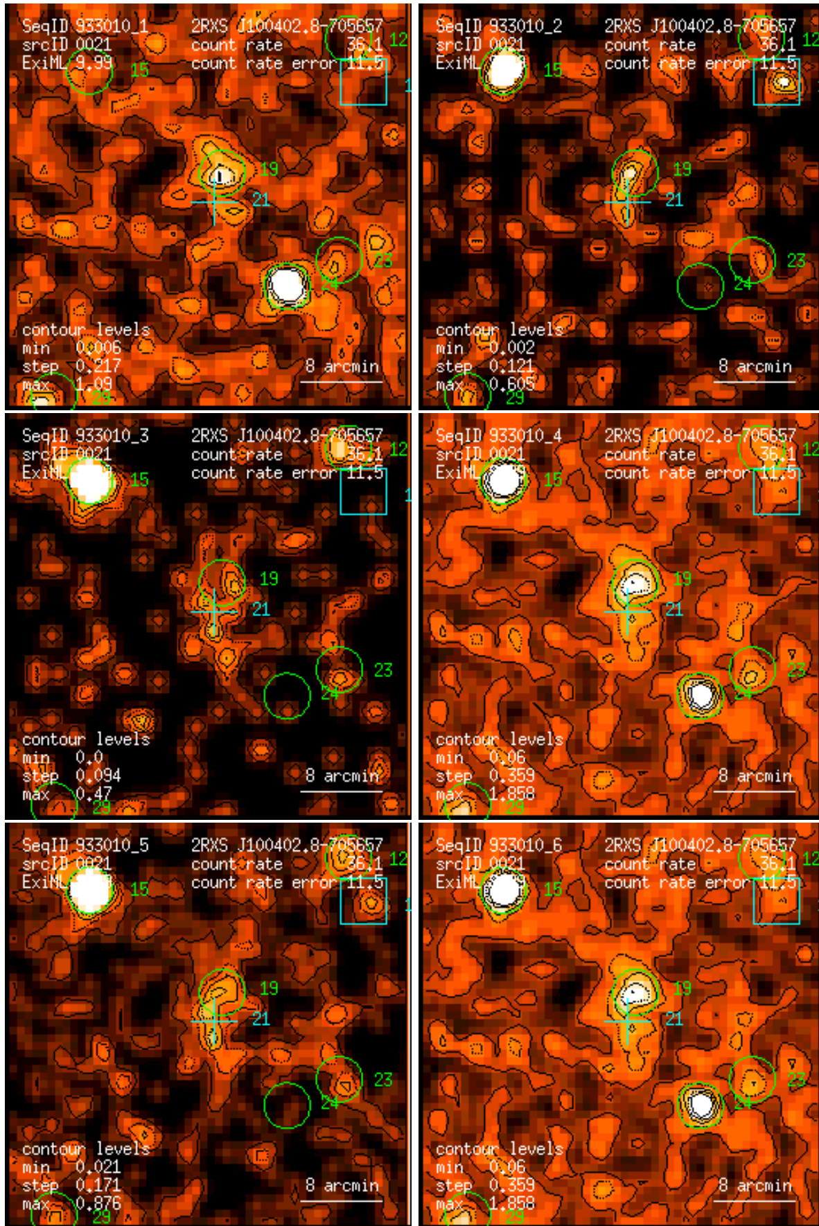
Figure 21: RASS 933010: detection 0021: band rate images, Gaussian filter: (1) PSPC channels 11 – 41, (2) 52 – 90, (3) 91 – 201, (4) 11 – 235, (5) 52 – 201, (6) 11 – 201. Broad band rates in counts/ks. Band rate contour levels in counts/ks/arcmin 2 .
