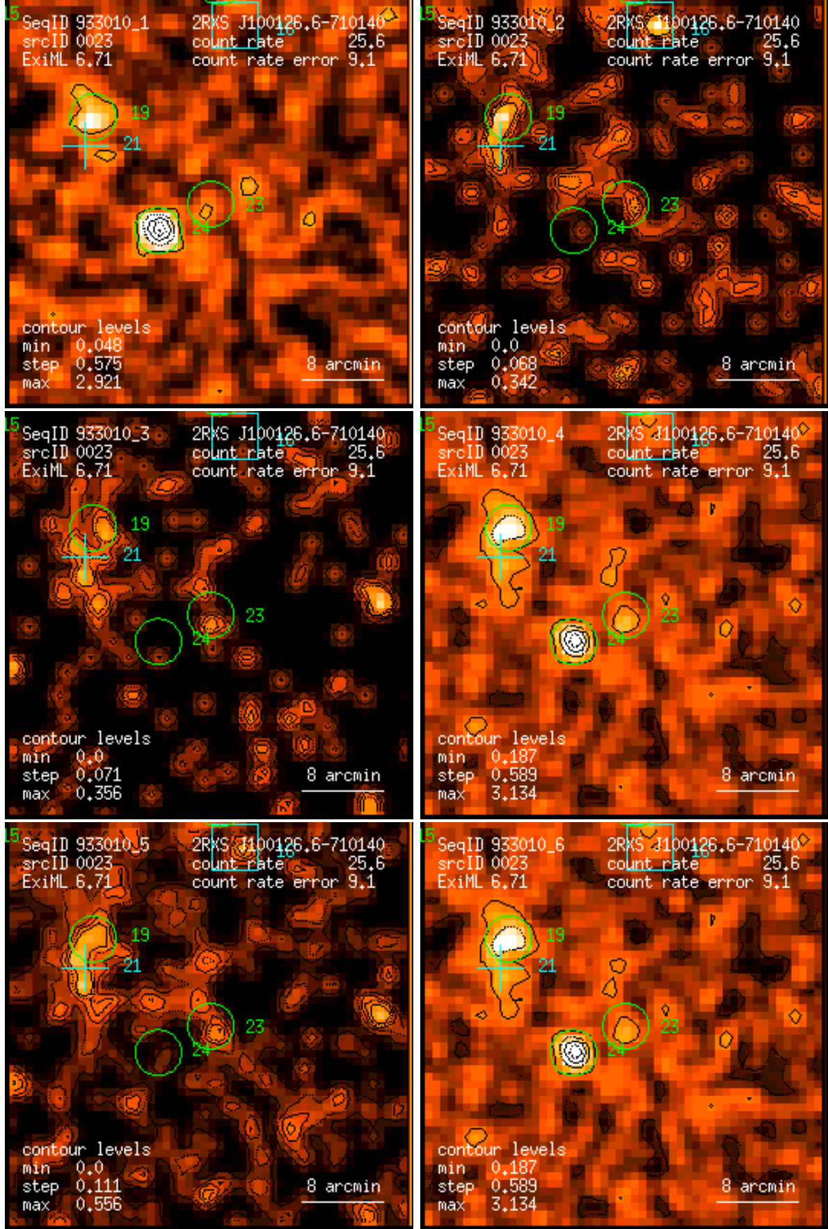
Figure 23: RASS 933010: detection 0023: band rate images, Gaussian filter: (1) PSPC channels 11 – 41, (2) 52 – 90, (3) 91 – 201, (4) 11 – 235, (5) 52 – 201, (6) 11 – 201. Broad band rates in counts/ks. Band rate contour levels in counts/ks/arcmin 2 .
