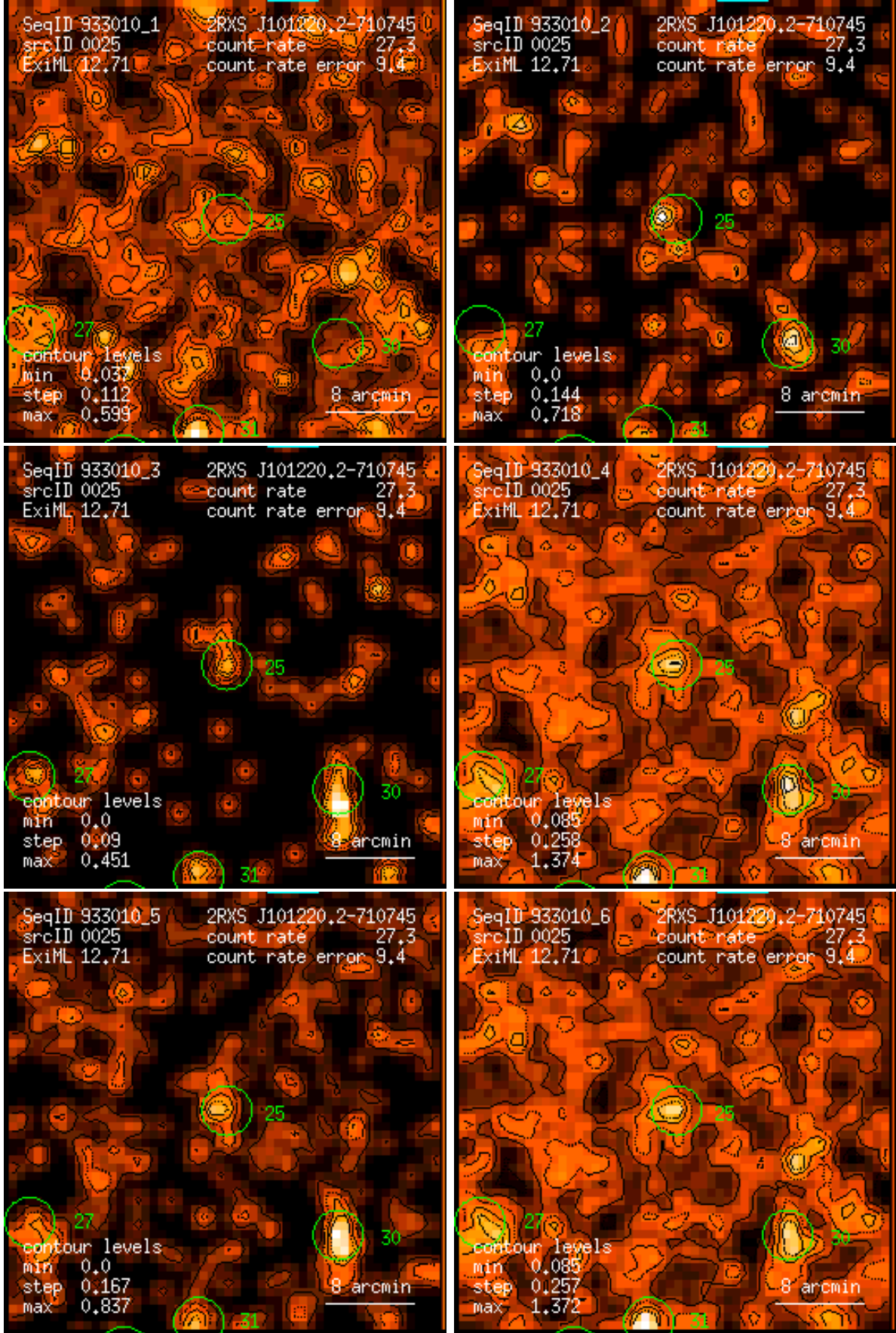
Figure 25: RASS 933010: detection 0025: band rate images, Gaussian filter: (1) PSPC channels 11 – 41, (2) 52 – 90, (3) 91 – 201, (4) 11 – 235, (5) 52 – 201, (6) 11 – 201. Broad band rates in counts/ks. Band rate contour levels in counts/ks/arcmin 2 .
