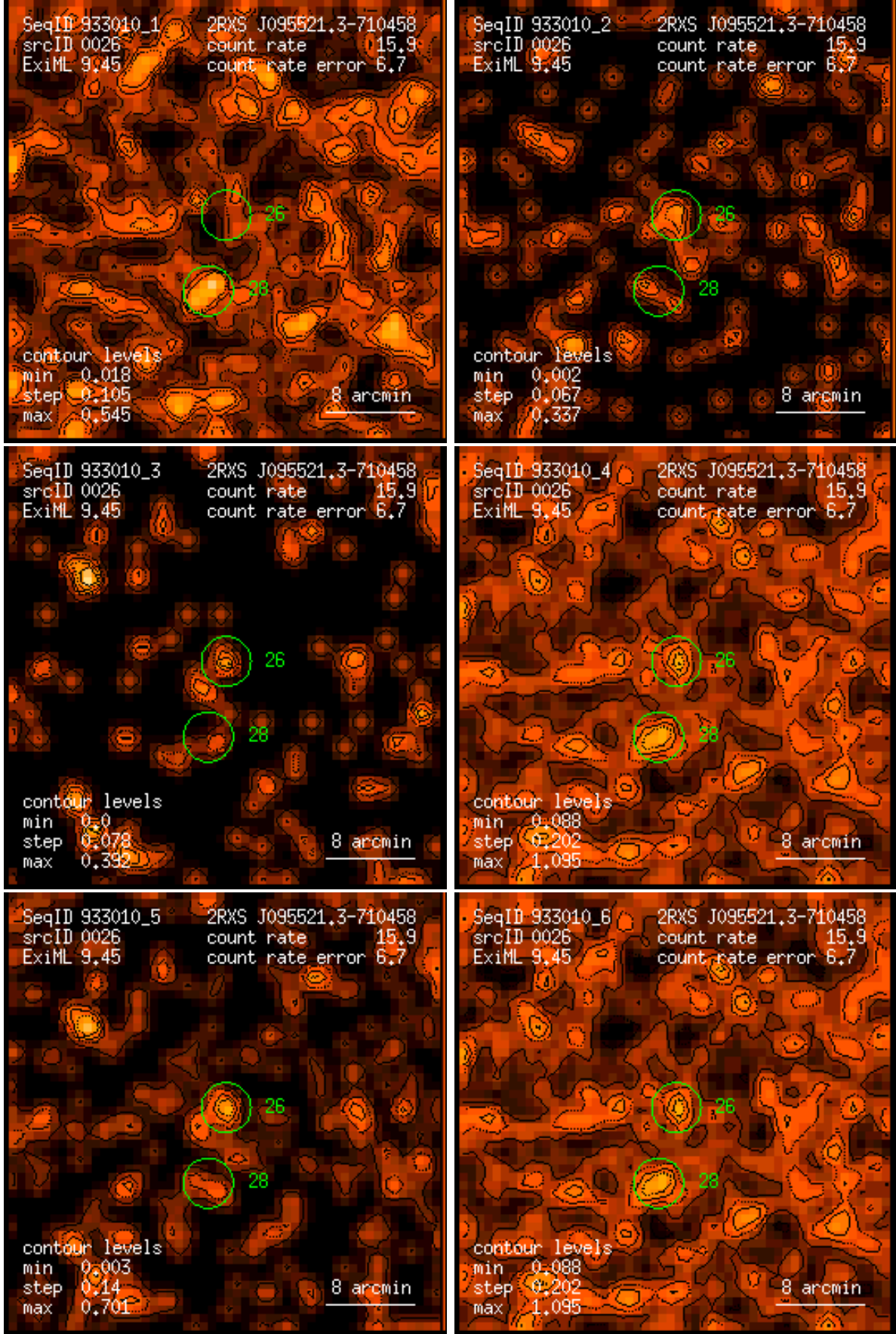
Figure 26: RASS 933010: detection 0026: band rate images, Gaussian filter: (1) PSPC channels 11 – 41, (2) 52 – 90, (3) 91 – 201, (4) 11 – 235, (5) 52 – 201, (6) 11 – 201. Broad band rates in counts/ks. Band rate contour levels in counts/ks/arcmin 2 .
