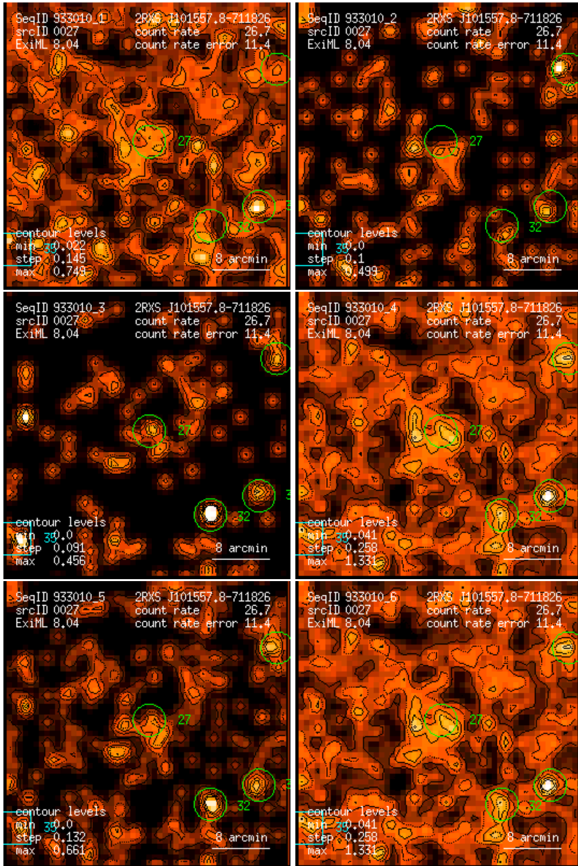
Figure 27: RASS 933010: detection 0027: band rate images, Gaussian filter: (1) PSPC channels 11 – 41, (2) 52 – 90, (3) 91 – 201, (4) 11 – 235, (5) 52 – 201, (6) 11 – 201. Broad band rates in counts/ks. Band rate contour levels in counts/ks/arcmin 2 .
