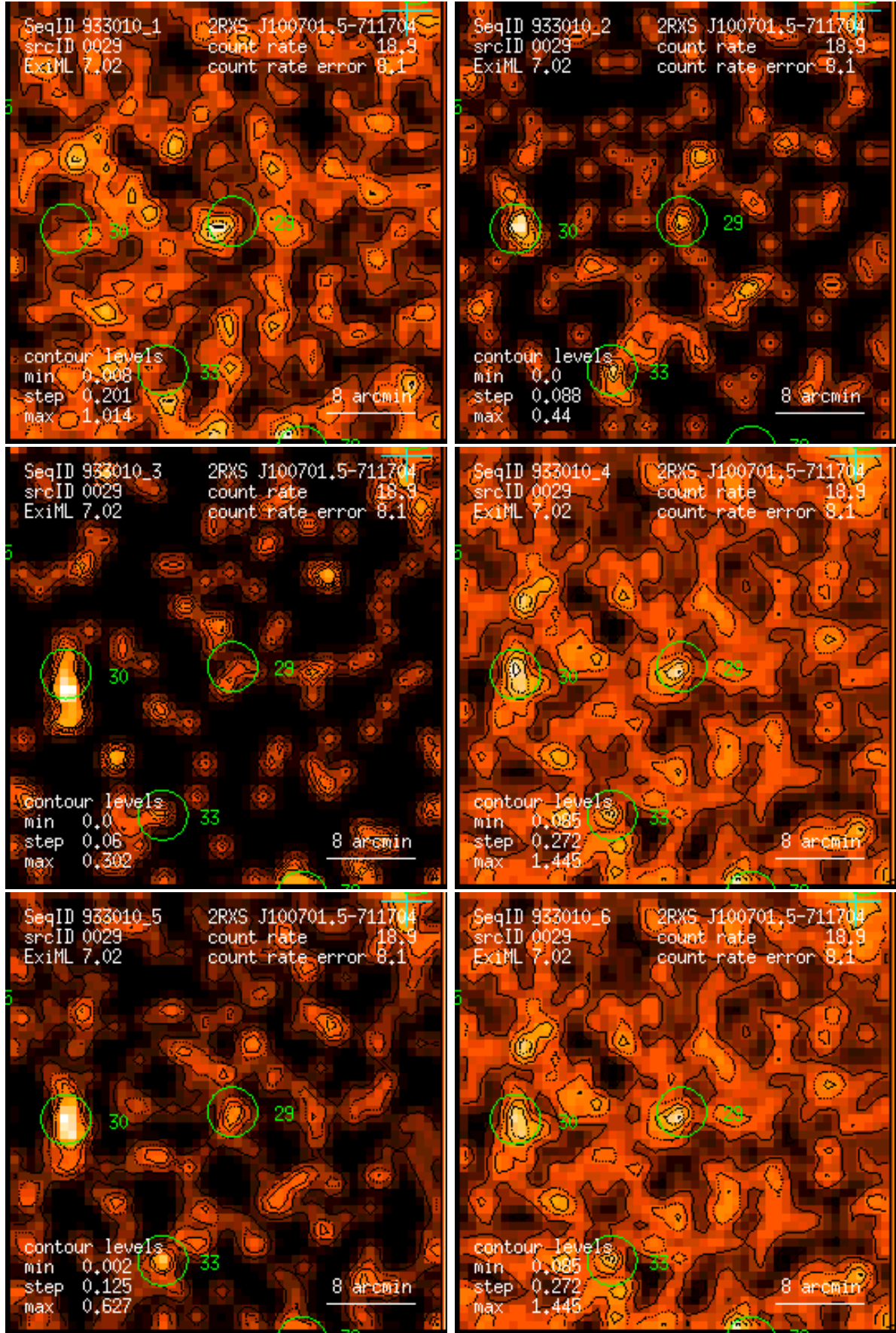
Figure 29: RASS 933010: detection 0029: band rate images, Gaussian filter: (1) PSPC channels 11 – 41, (2) 52 – 90, (3) 91 – 201, (4) 11 – 235, (5) 52 – 201, (6) 11 – 201. Broad band rates in counts/ks. Band rate contour levels in counts/ks/arcmin 2 .
