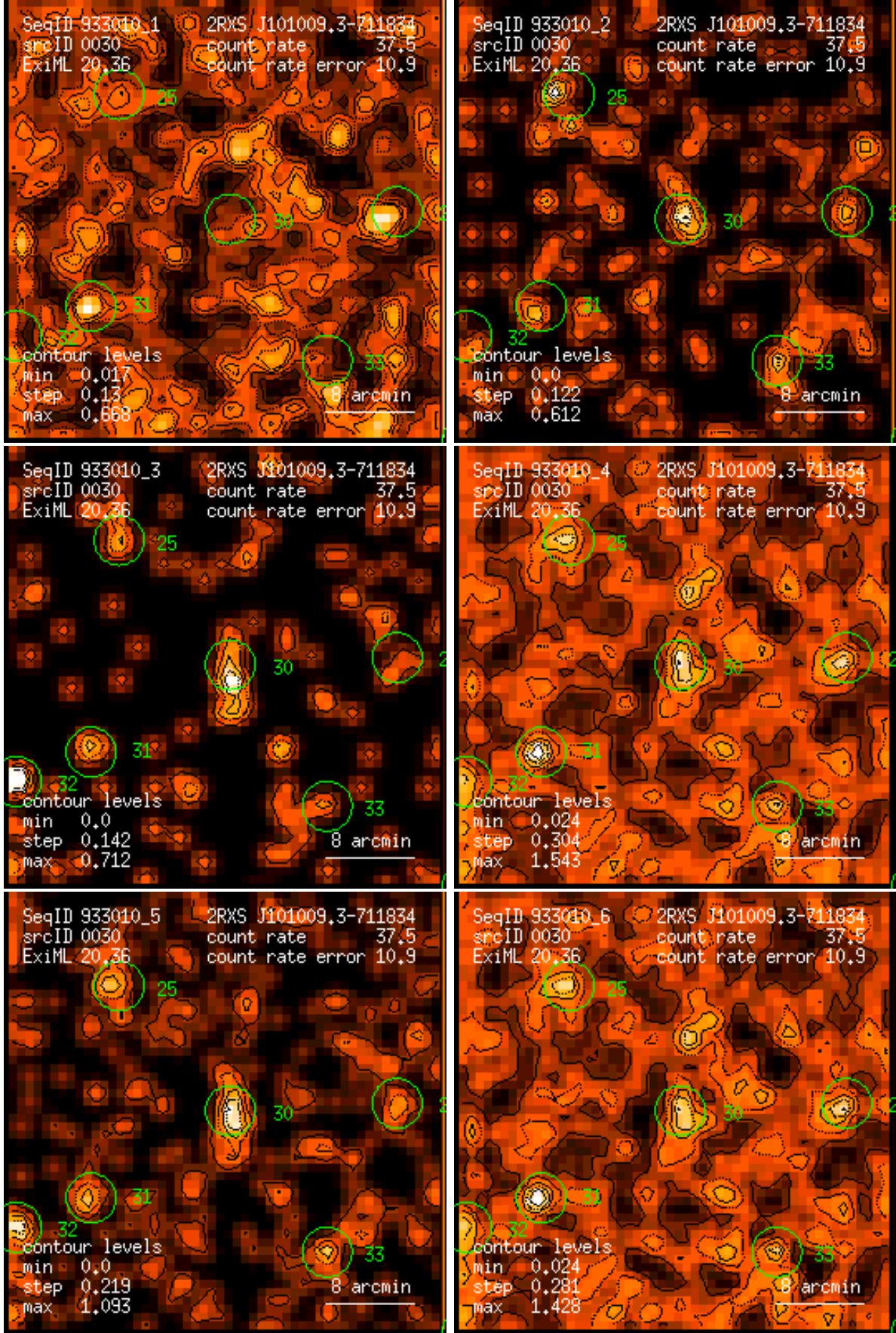
Figure 30: RASS 933010: detection 0030: band rate images, Gaussian filter: (1) PSPC channels 11 – 41, (2) 52 – 90, (3) 91 – 201, (4) 11 – 235, (5) 52 – 201, (6) 11 – 201. Broad band rates in counts/ks. Band rate contour levels in counts/ks/arcmin 2 .
