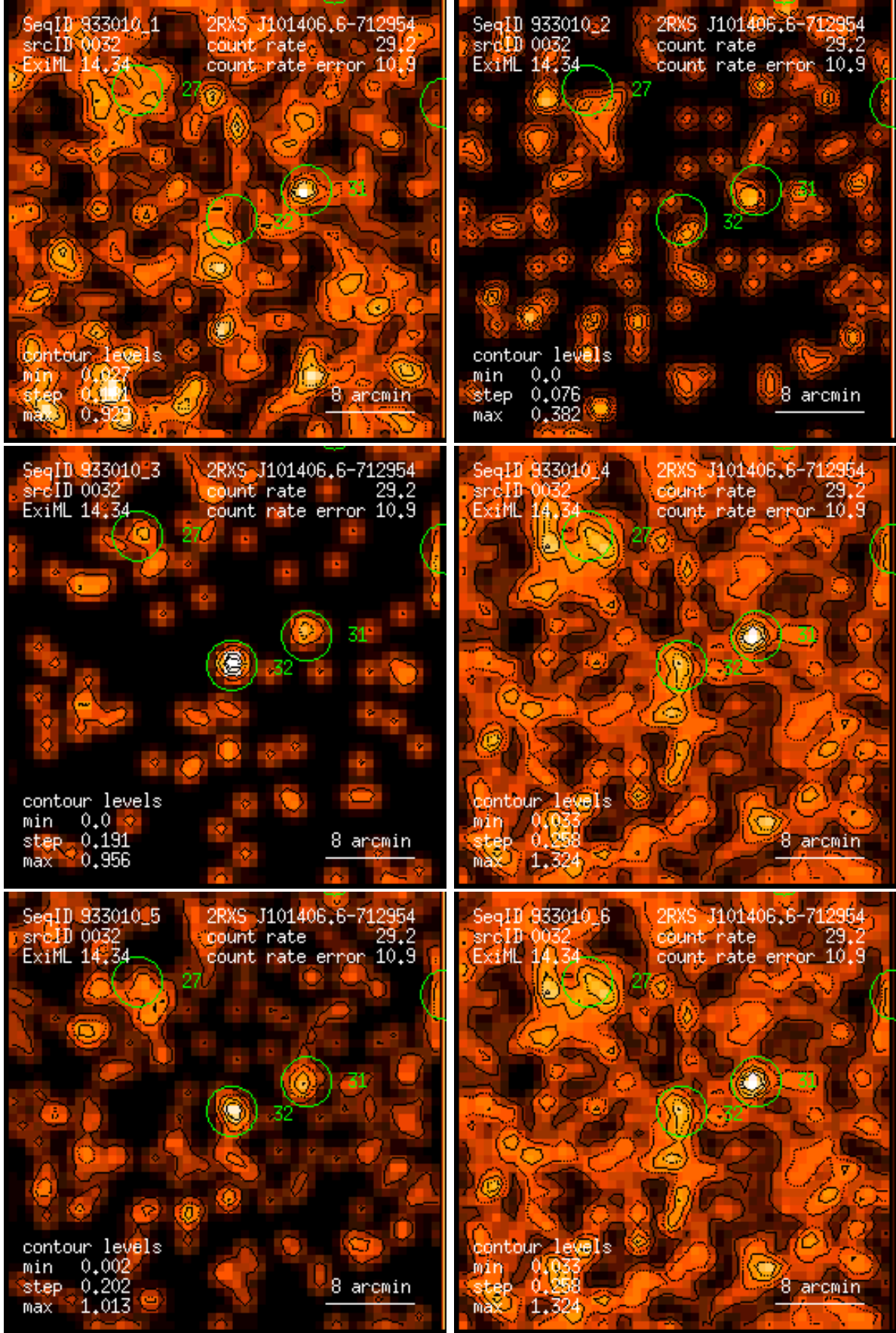
Figure 32: RASS 933010: detection 0032: band rate images, Gaussian filter: (1) PSPC channels 11 – 41, (2) 52 – 90, (3) 91 – 201, (4) 11 – 235, (5) 52 – 201, (6) 11 – 201. Broad band rates in counts/ks. Band rate contour levels in counts/ks/arcmin 2 .
