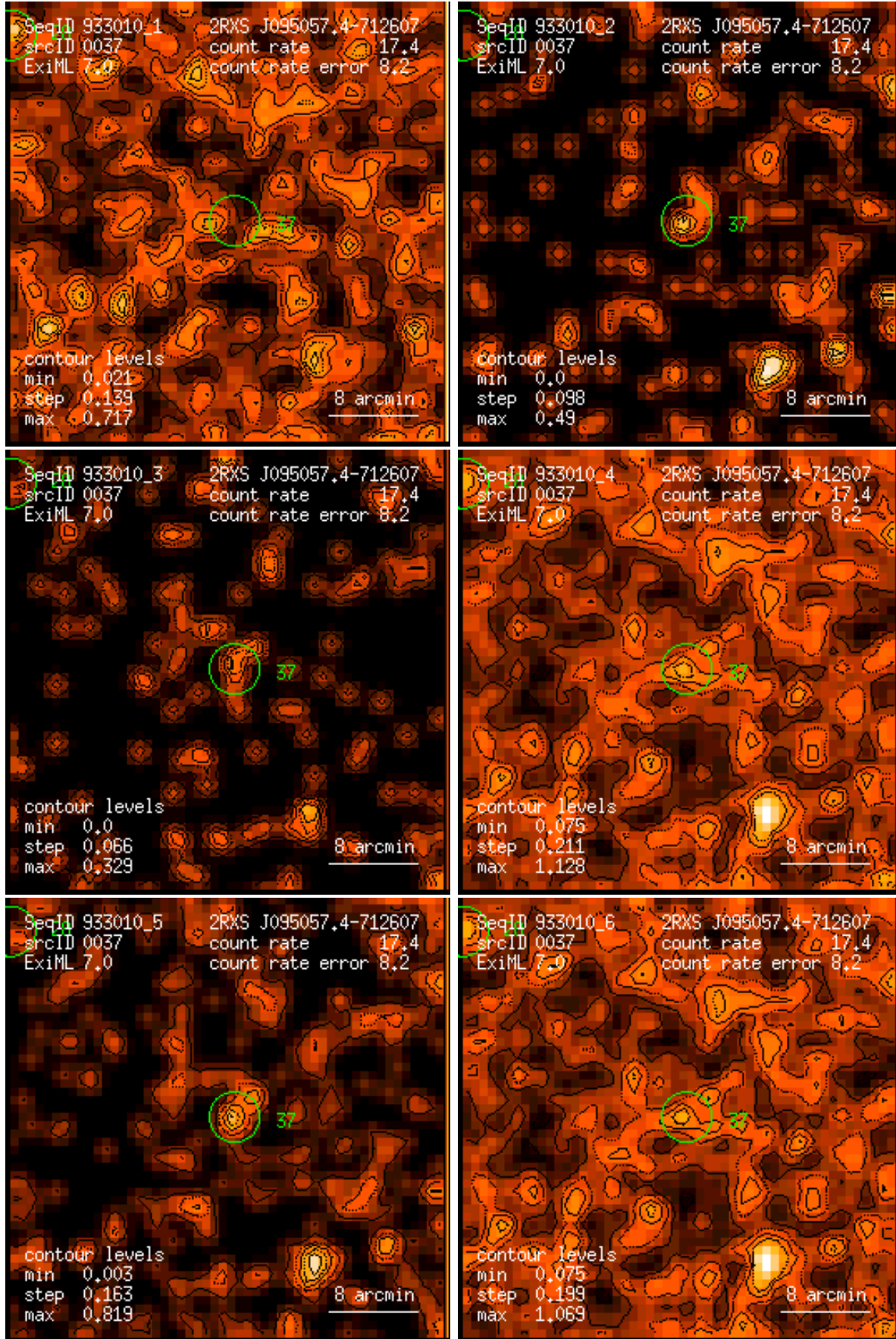
Figure 37: RASS 933010: detection 0037: band rate images, Gaussian filter: (1) PSPC channels 11 – 41, (2) 52 – 90, (3) 91 – 201, (4) 11 – 235, (5) 52 – 201, (6) 11 – 201. Broad band rates in counts/ks. Band rate contour levels in counts/ks/arcmin 2 .
