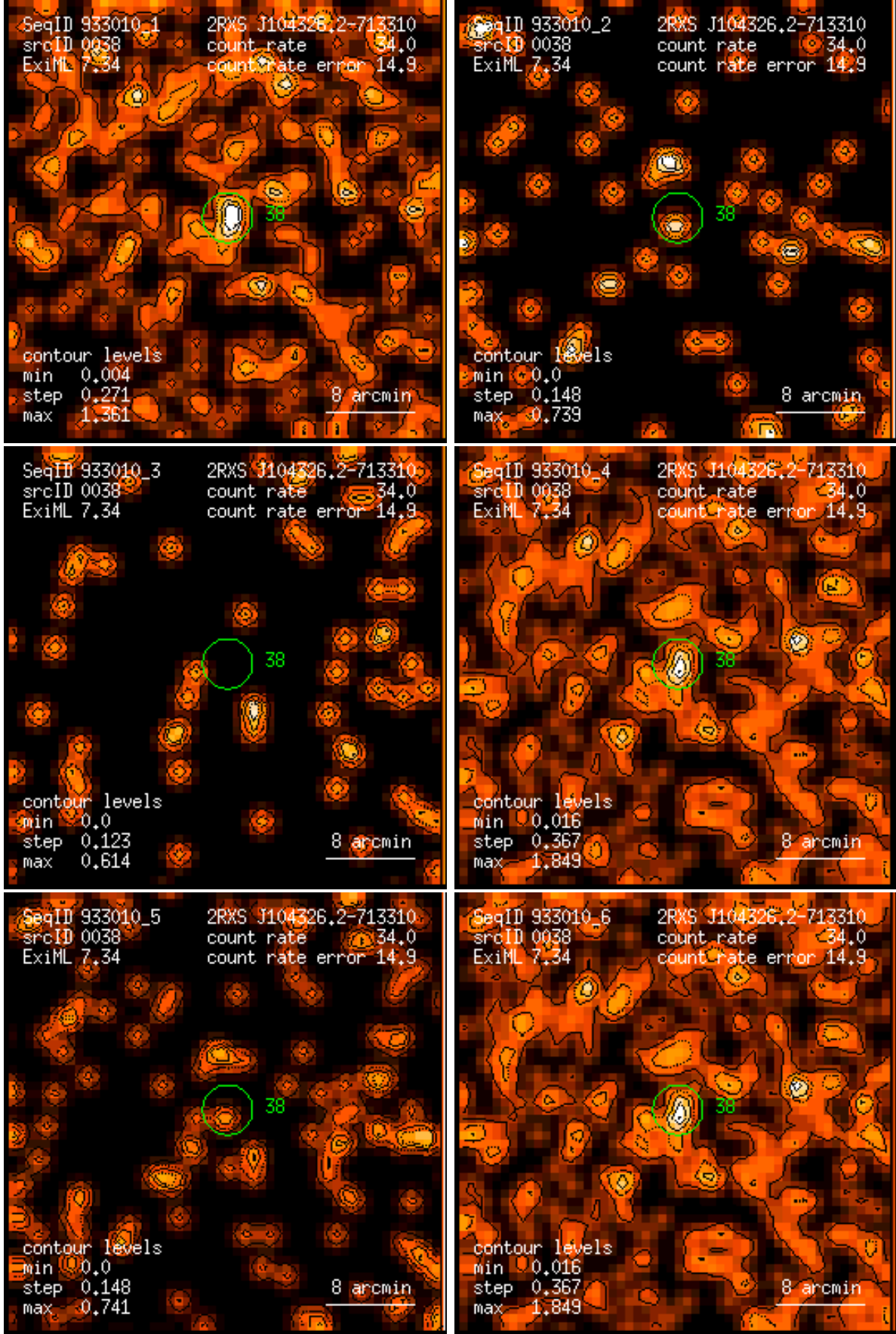
Figure 38: RASS 933010: detection 0038: band rate images, Gaussian filter: (1) PSPC channels 11 – 41, (2) 52 – 90, (3) 91 – 201, (4) 11 – 235, (5) 52 – 201, (6) 11 – 201. Broad band rates in counts/ks. Band rate contour levels in counts/ks/arcmin 2 .
