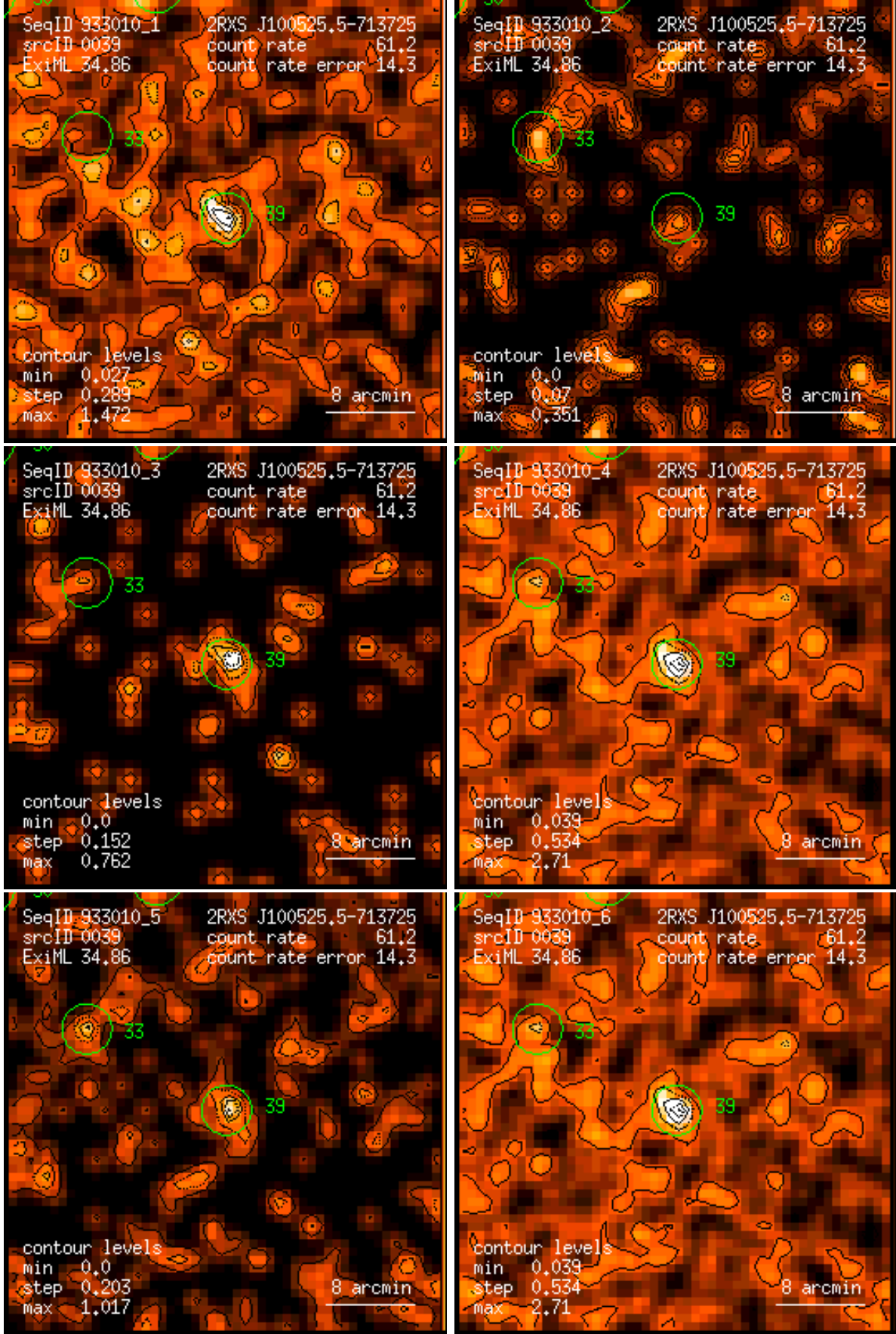
Figure 39: RASS 933010: detection 0039: band rate images, Gaussian filter: (1) PSPC channels 11 – 41, (2) 52 – 90, (3) 91 – 201, (4) 11 – 235, (5) 52 – 201, (6) 11 – 201. Broad band rates in counts/ks. Band rate contour levels in counts/ks/arcmin 2 .
