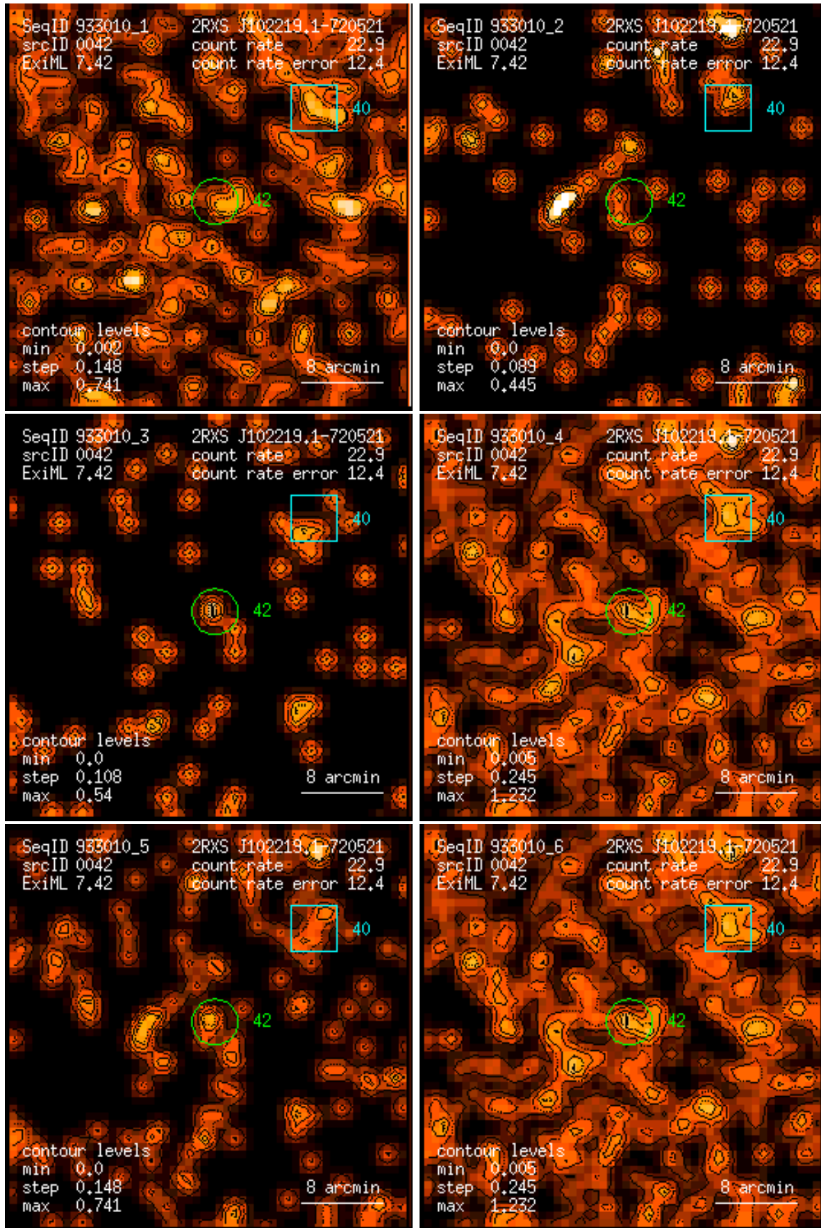
Figure 42: RASS 933010: detection 0042: band rate images, Gaussian filter: (1) PSPC channels 11 – 41, (2) 52 – 90, (3) 91 – 201, (4) 11 – 235, (5) 52 – 201, (6) 11 – 201. Broad band rates in counts/ks. Band rate contour levels in counts/ks/arcmin 2 .
