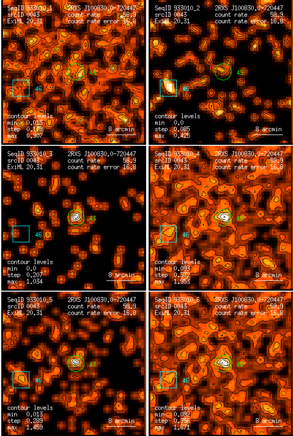
Figure 43: RASS 933010: detection 0043: band rate images, Gaussian filter: (1) PSPC channels 11 – 41, (2) 52 – 90, (3) 91 – 201, (4) 11 – 235, (5) 52 – 201, (6) 11 – 201. Broad band rates in counts/ks. Band rate contour levels in counts/ks/arcmin 2 .
