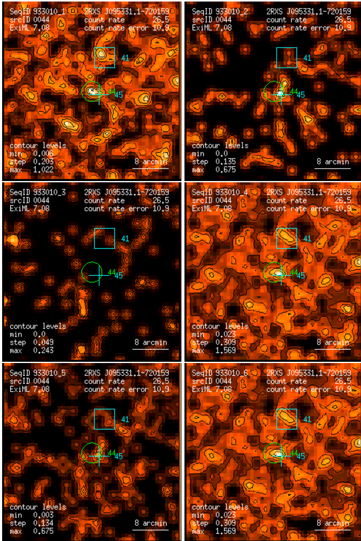
Figure 44: RASS 933010: detection 0044: band rate images, Gaussian filter: (1) PSPC channels 11 – 41, (2) 52 – 90, (3) 91 – 201, (4) 11 – 235, (5) 52 – 201, (6) 11 – 201. Broad band rates in counts/ks. Band rate contour levels in counts/ks/arcmin 2 .
