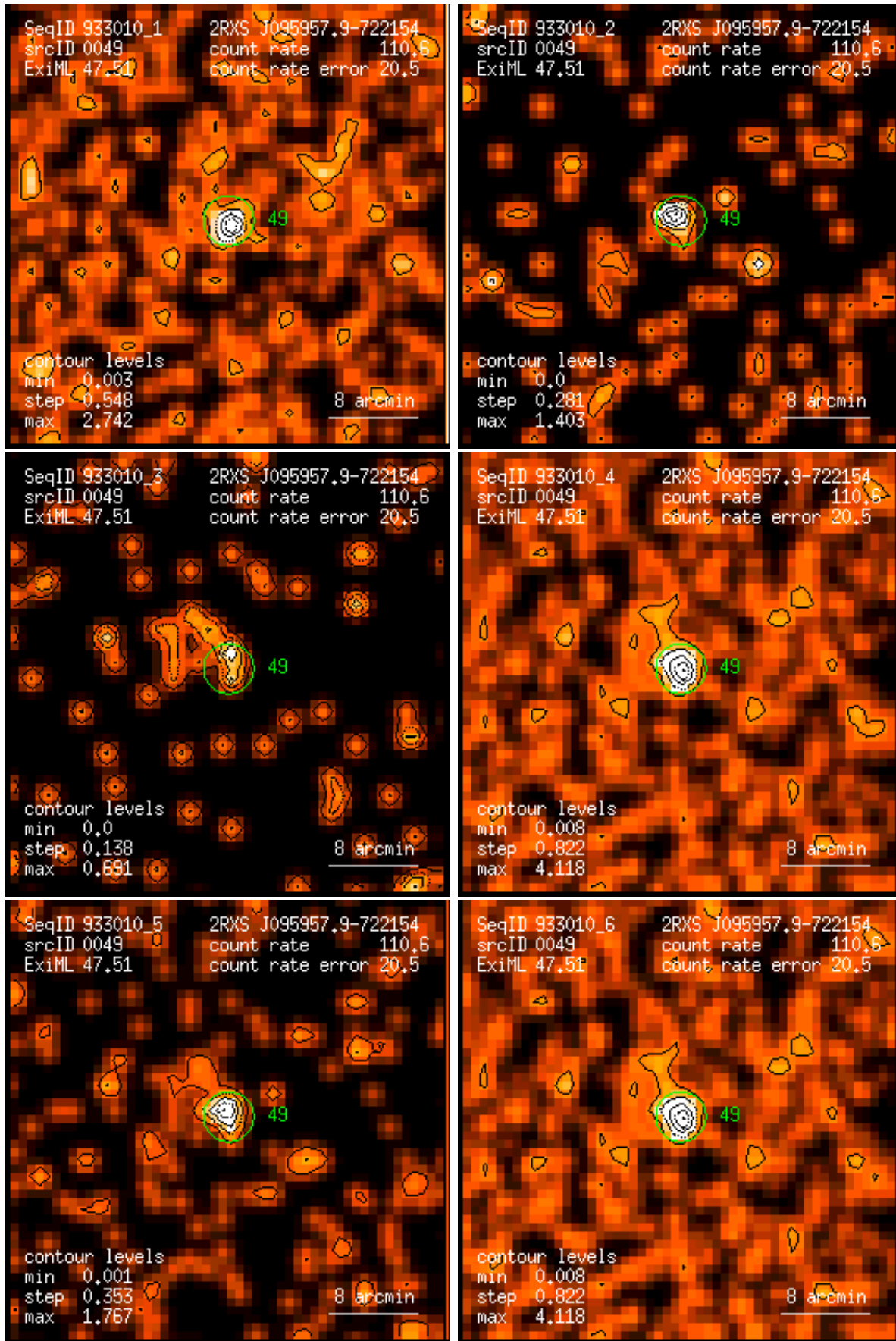
Figure 49: RASS 933010: detection 0049: band rate images, Gaussian filter: (1) PSPC channels 11 – 41, (2) 52 – 90, (3) 91 – 201, (4) 11 – 235, (5) 52 – 201, (6) 11 – 201. Broad band rates in counts/ks. Band rate contour levels in counts/ks/arcmin 2 .
