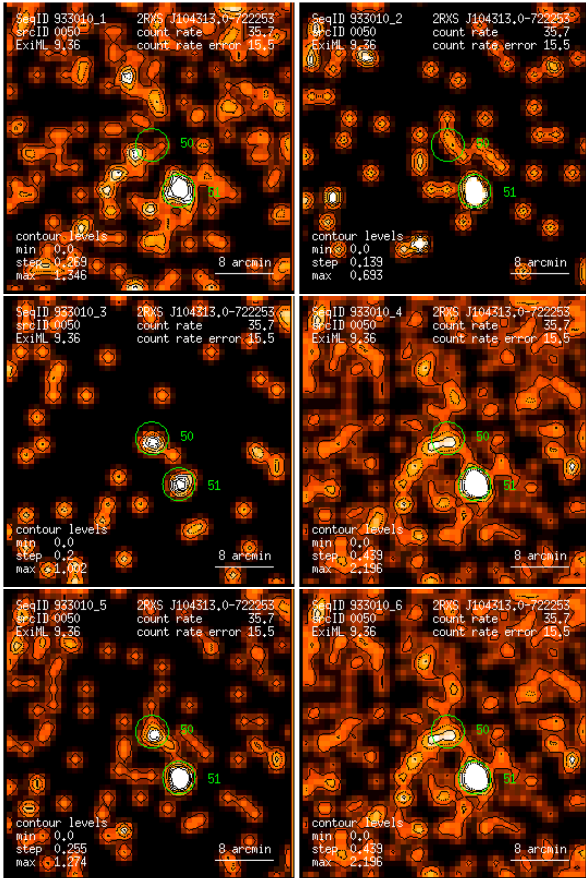
Figure 50: RASS 933010: detection 0050: band rate images, Gaussian filter: (1) PSPC channels 11 – 41, (2) 52 – 90, (3) 91 – 201, (4) 11 – 235, (5) 52 – 201, (6) 11 – 201. Broad band rates in counts/ks. Band rate contour levels in counts/ks/arcmin 2 .
