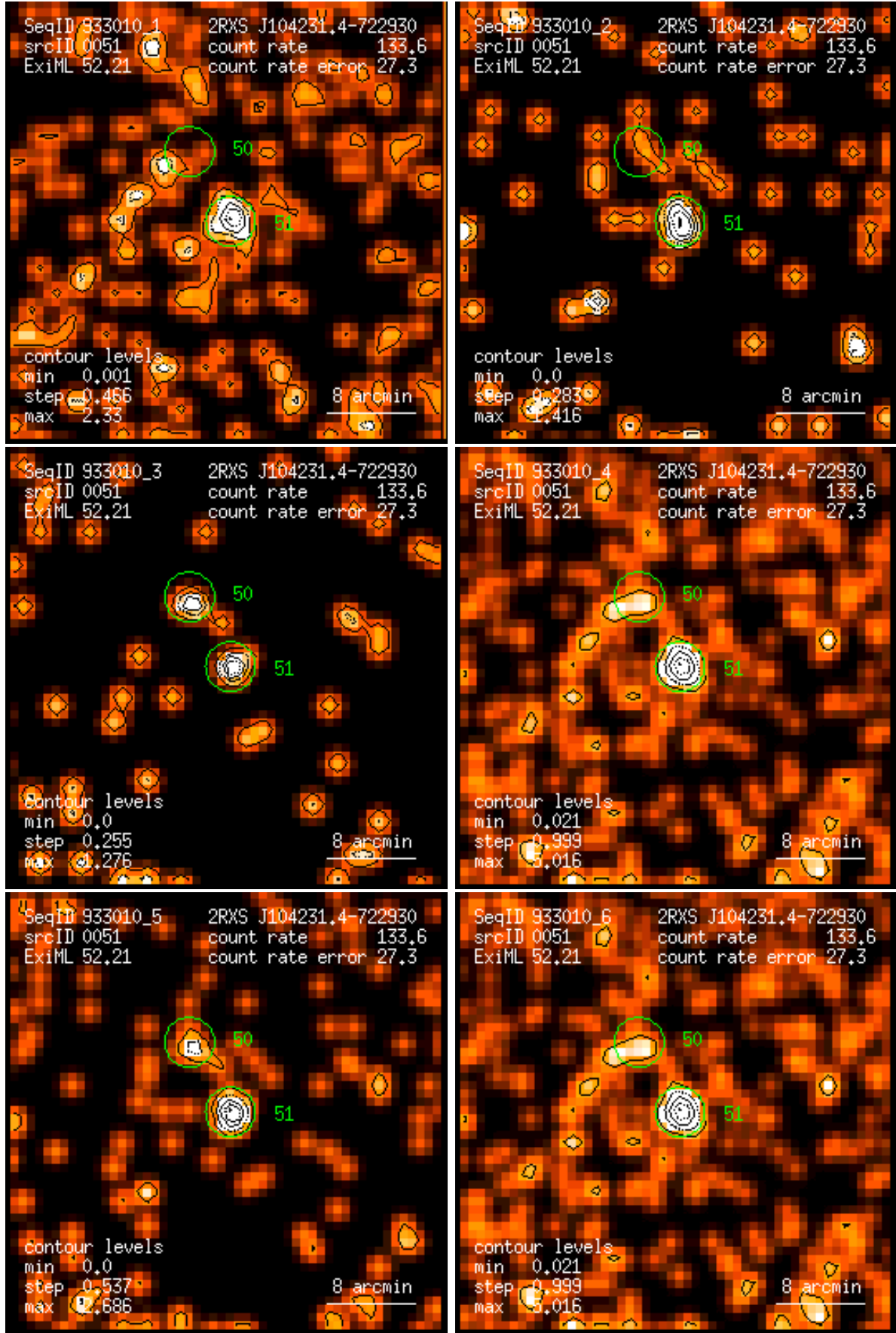
Figure 51: RASS 933010: detection 0051: band rate images, Gaussian filter: (1) PSPC channels 11 – 41, (2) 52 – 90, (3) 91 – 201, (4) 11 – 235, (5) 52 – 201, (6) 11 – 201. Broad band rates in counts/ks. Band rate contour levels in counts/ks/arcmin 2 .
