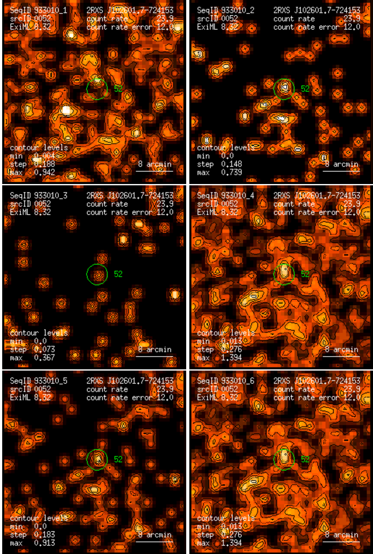
Figure 52: RASS 933010: detection 0052: band rate images, Gaussian filter: (1) PSPC channels 11 – 41, (2) 52 – 90, (3) 91 – 201, (4) 11 – 235, (5) 52 – 201, (6) 11 – 201. Broad band rates in counts/ks. Band rate contour levels in counts/ks/arcmin 2 .
